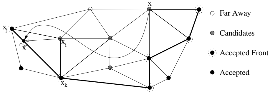
Figure 4.3: The AcceptedFront and the Considered mesh points. The optimal trajectory for \bar{\mathbf{x}} cannot intersect AF too far away from \bar{\mathbf{x}} , for if \|\tilde{\mathbf{x}} - \bar{\mathbf{x}}\| > h\frac{F_2}{F_1} , then u(\mathbf{x}_i) < u(\bar{\mathbf{x}}) .
