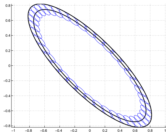
Fig.6.5B: modified Huygens' construction for an expanding ellipse.
