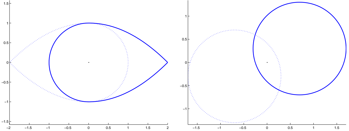
Figure 6.1: Two examples of vehicle's speed profiles \rho = f(\theta) . The dotted line shows the “flipped” version of the profile, i.e., \rho = g(\theta) = f(\theta + \pi) .
