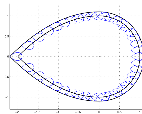
Fig.6.5D: modified Huygens' construction for an expanding droplet.
