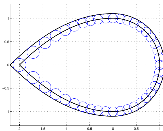
Fig.6.5C: canonical Huygens' construction for an expanding droplet.
