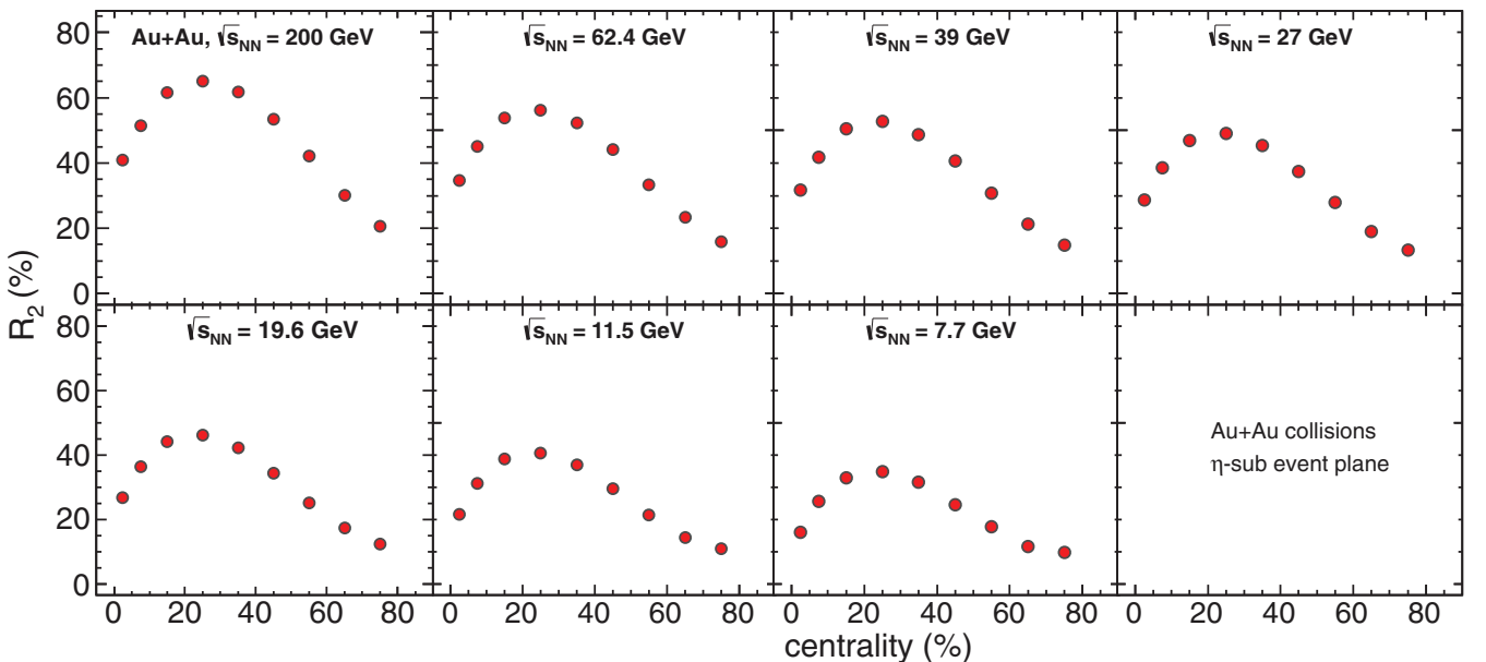
FIG. 2. Resolution correction factor R_2 of subevent planes as a function of centrality for Au + Au collisions at \sqrt{s_{NN}} = 200, 62.4, 39, 27, 19.6, 11.5, \text{ and } 7.7 GeV.
