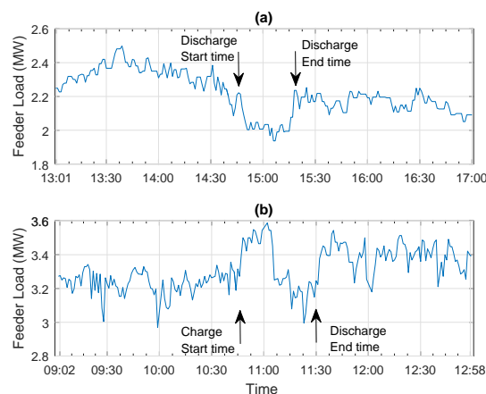
Fig. 8. Battery signatures at Feeder #1224 on 4/23 and 9/11.
