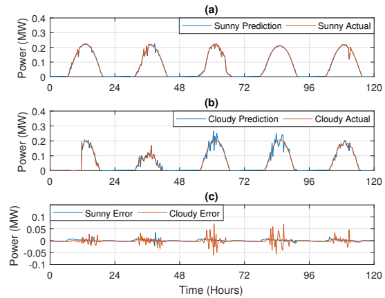
Fig. 6. The results on separate solar generation forecast: (a) Actual and predicted solar output for a sunny week; (b) actual and predicted solar output for a cloudy week; (c) estimation error for both the sunny and cloudy forecasts
