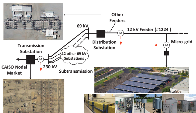
Fig. 1. A wide view of the overall utility-scale test system in this study.
