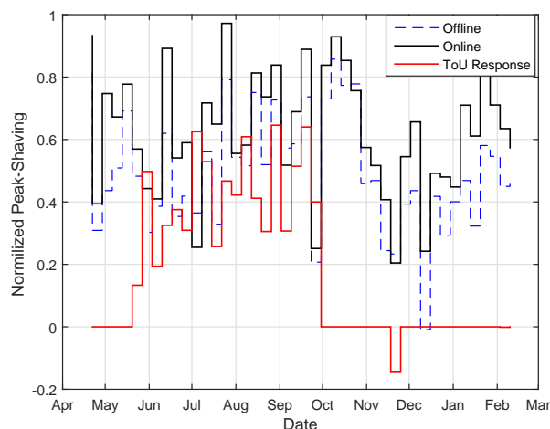
Fig. 12. The weekly normalized amount of peak load shaving achieved on the feeder by operating the battery system based on responding to ToU pricing, offline stochastic optimization, and online stochastic optimization.
