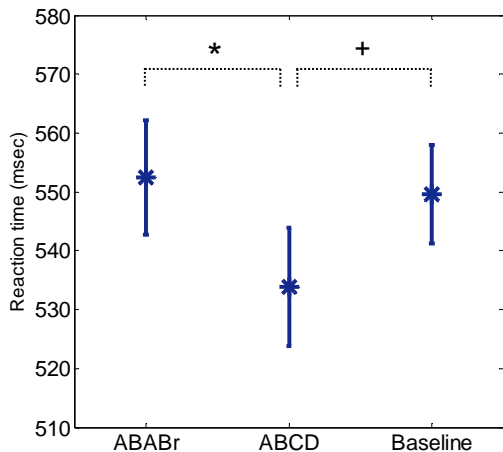
Figure 6: Comparing the asymptotic point for each condition during learning. Error bars indicate +/- one standard error. * indicates p < .05 , + indicates p = .10
