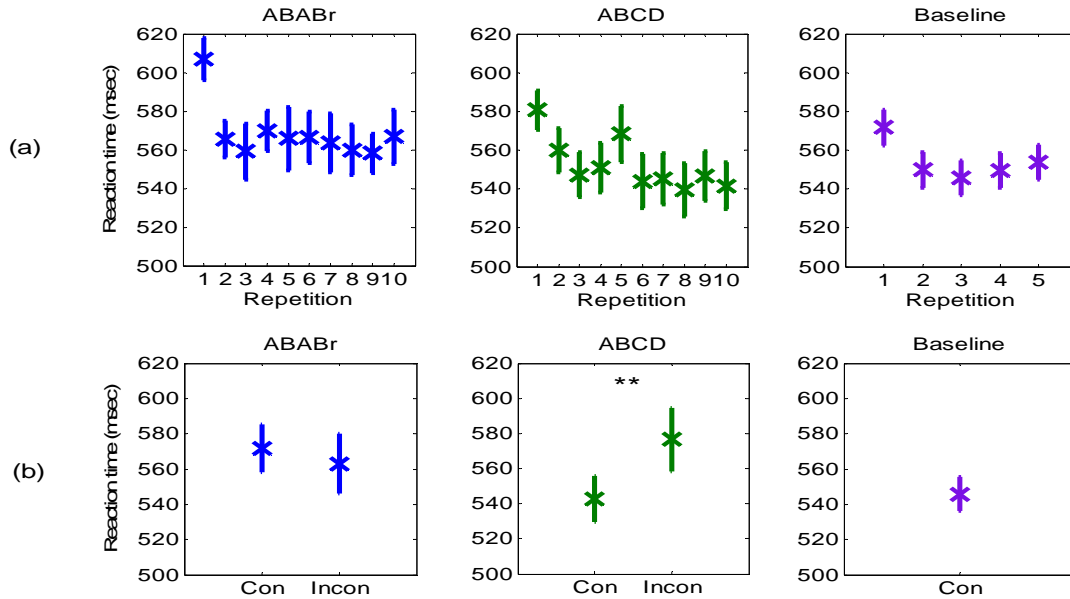
Figure 5: RT at each condition during (a) learning at each repetition, (b) test at congruent (Con) and incongruent (Incon) trials. Error bars indicate +/- one standard error. ** indicates p < .005 .
