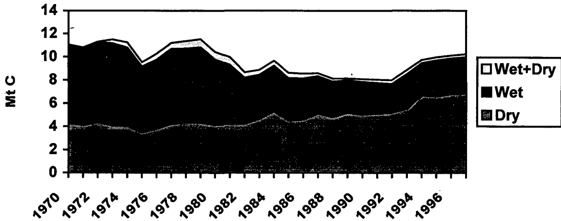
Figure 5. Carbon Emissions from the U.S. Cement Industry by Clinker Production Process, 1970 to 1997 (expressed in Mt C/year). Source: USGS, various years.
