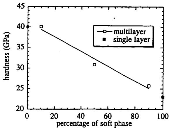
Fig. 4 Peak hardness of single layers of soft and hard carbon in comparison to multilayer structures containing soft and hard carbon layers in different thickness ratios.
