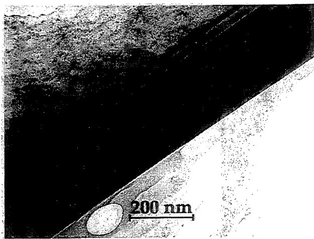
Fig. 6 TEM cross-section image of hard phase/soft phase amorphous carbon multilayer on silicon. Top left - silicon substrate, bottom right - glue for sample preparation.
