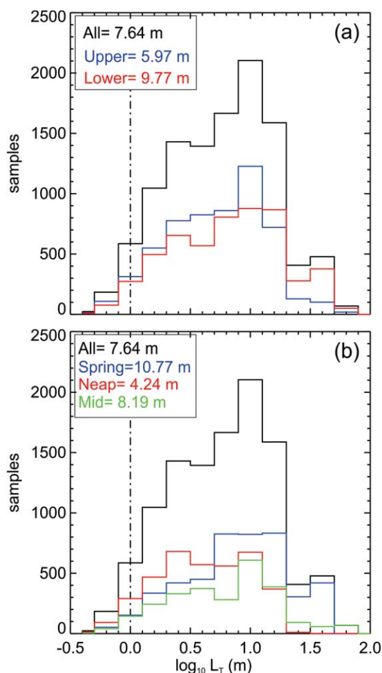
Figure 15. Distributions of Thorpe Scale L_T derived from scalar sensors on the VMP profiler showing separation based on (a) depth in the water column (upper <130 m) and (b) tidal spring-neap phase. In both plots, the total distribution is shown in black. The vertical dashed line at \log_{10}(L_T) = 0 (i.e., 1 m) is a cutoff whereby samples to the left are likely unreliable due to sampling limitations.
