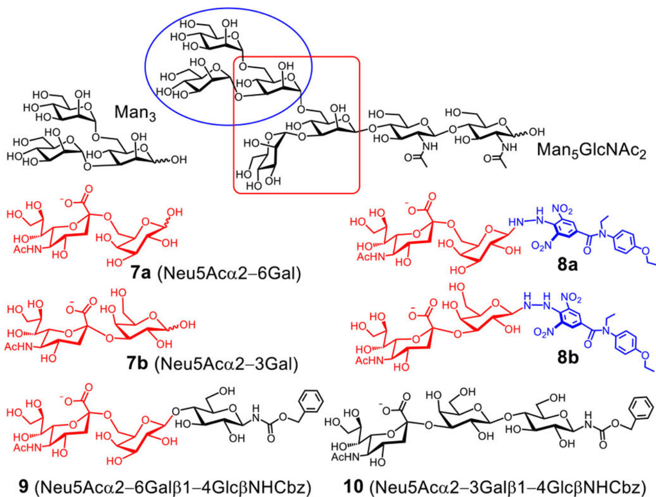
Figure 1. Structures of key glycans used in this work.
