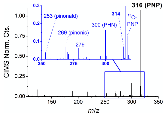
Figure 4. Negative ion CIMS mass spectrum after 1 h of oxidation under simulated nighttime conditions, showing PNP, PHN, and another organic nitrogen product at m/z 314. Pinonaldehyde is observed at m/z 253 and pinonic acid at m/z 269.
