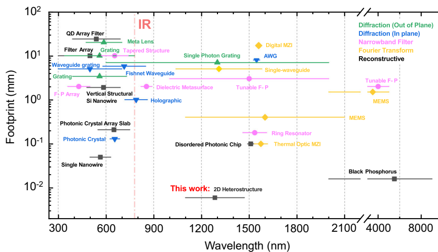
Fig. 6 | Plot of comparison between this work and other reported works for the key parameter footprint and spectral range. Five types of system are divided according to their operational mechanism 3 , including out of plane diffraction, in plane diffraction, narrowband filter, Fourier Transform, and reconstructive. The
