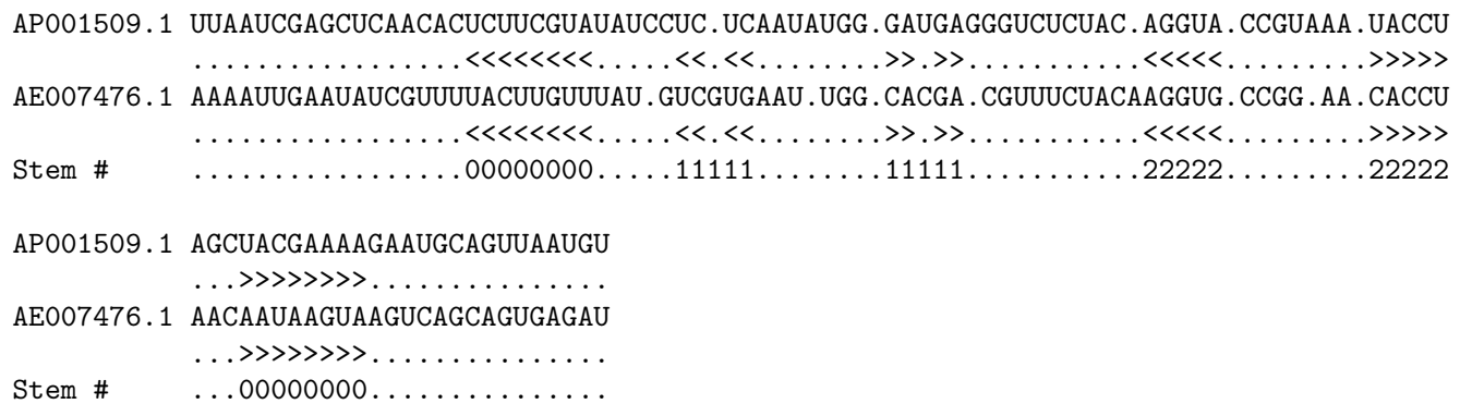
Figure 9 Alignment of purine riboswitches from Bacillus halodurans (AP001509.1) and Streptococcus pneumoniae (AE007476.1).
