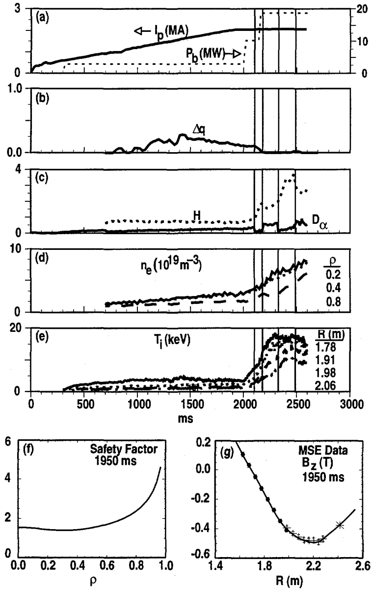
Fig. 1. (a) Early beam power during the current ramp produces the NCS configuration. (b) This double-null plasma (87935) has weak shear [ \Delta q = q(0) - q_{min} ]. (c) There are two H-mode edge phases (divertor D_{\alpha} emission) in this discharge marked by the vertical lines. Enhancement ( H ) over ITER-89P exceeds 3. (d) Density profiles are peaked in L-mode edge and broad in H-mode edge. (e) Ion temperature is more peaked in L-mode edge. (f,g) The MSE diagnostic measures the local magnetic field pitch angle and, combined with magnetic probe measurements, results in a well determined q profile.
