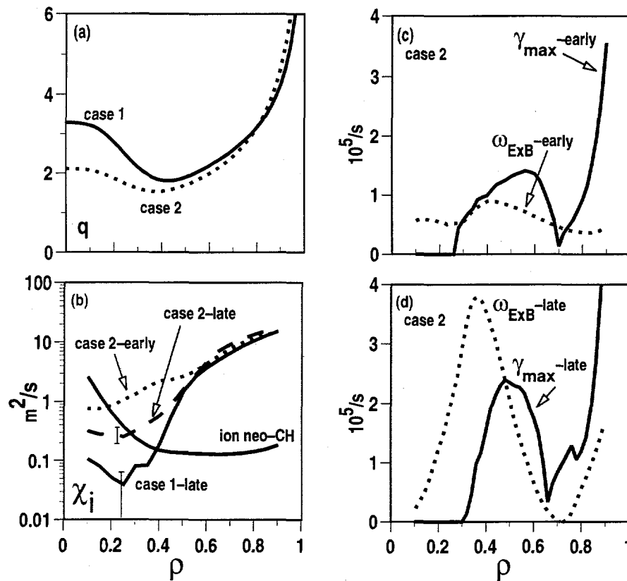
Fig. 5. (a) L-mode edge NCS plasmas with larger negative magnetic shear (Case 1 - 87003) and weak shear (Case 2 - 87031). (b) \chi_i is reduced from before (early at 5 MW) the transport barrier to after (late at 10 MW) the transport barrier formation. For fixed conditions \chi_i is reduced for larger magnetic shear. (c) During the early formation of the transport barrier the turbulence growth rate ( \gamma_{\max} ) exceeds the Doppler shift shear rate ( \omega_{\text{ExB}} ). (d) After the transport barrier formation \gamma_{\max} < \omega_{\text{ExB}} in the region of reduced ion transport.
