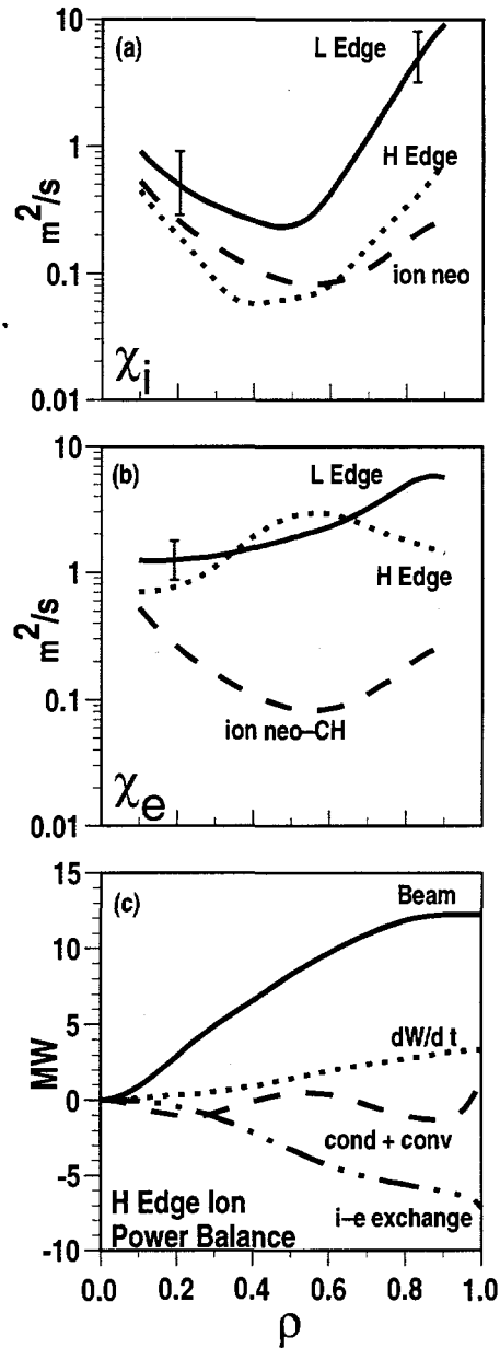
Fig. 3. (a, b) Ion and electron diffusivity for the NCS discharge (87935) of Fig. 1. The L-mode edge time is taken at 2.3 s and the H-mode edge time 2.45 s. The NCS H-mode edge \chi_i is near neoclassical over the entire cross section. (c) The NCS H-mode edge ion power balance shows both conduction and convection are reduced to a negligible level.
