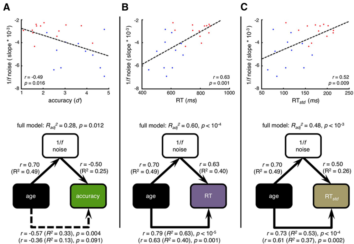
Figure 4. 1/f noise and behavior. A , Greater visual cortical 1/f noise across younger (blue) and older (red) adults predicts lower working memory performance (top). Mediation analyses (bottom) shows that visual cortical 1/f noise statistically mediates age-related visual working memory decline. Although aging is associated with both increased 1/f noise and decreased visual working memory accuracy, and visual cortical 1/f noise predicts accuracy impairments, the relationship between age and accuracy became insignificant after including 1/f noise in the model (bottom r/p value pairs). 1/f noise is also associated with longer RTs ( B ) and greater RT variability ( C ); however, it does not act as a mediating variable for either of these RT measures.
