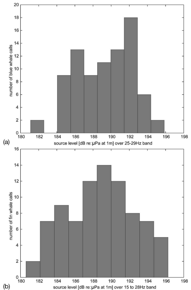
FIG. 5. Distribution of (a) blue whale call source levels, with the mean of 189 \pm 3 dB re : 1 \mu Pa at 1 m over the 25–29-Hz band ( N=84 ) and (b) fin whale call source levels, with the mean of 189 \pm 4 dB re : 1 \mu Pa at 1 m over the 15–28-Hz band ( N=83 ).
