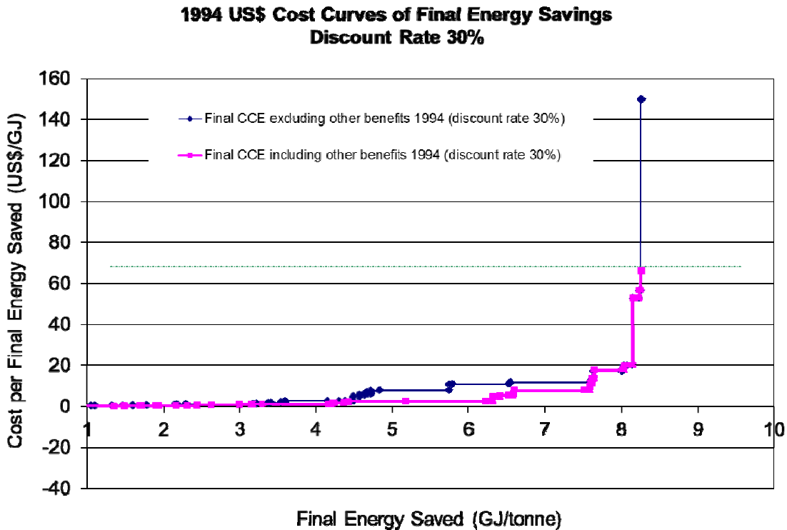
Figure 3. Cost curves for inclusion and exclusion of other benefits in the U.S. iron and steel industry
