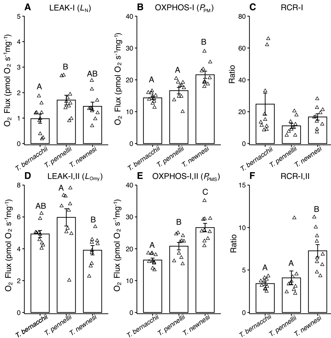
Fig. 1 Mitochondrial respiration during LEAK and OXPPOS states in permeabilized ventricle fibers of adult Trematomus bernacchii , T. pennellii and T. newnesi . There was a significant effect of species on A LEAK-I respiration ( L_N ; ANOVA; F_{(2,27)}=4.3 , P=0.04 ) and B OXPPOS-I respiration measured with maximal ADP and substrates of complex I ( P_{PM} ; ANOVA; F_{(2,27)}=16.1 , P<0.01 ). There was no effect of species on C respiratory control ratio RCR-I ( P_{PM}/L_N ; ANOVA; F_{(2,27)}=3.0 , P=0.14 ). There was a signifi-
