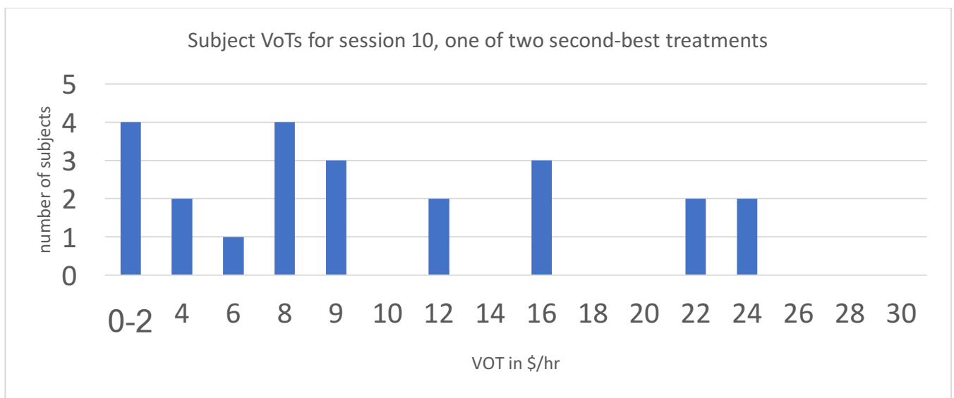
Figure 31: Distribution of Subjects' Average VOT Elicited from a Second-best VCG Mechanism
