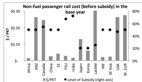
Figure 9.1: Non-fuel passenger rail cost (before subsidy) in 2005
