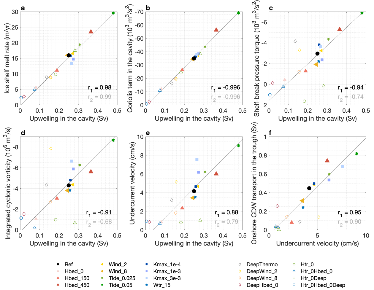
Figure 4.5: Perturbation experiments. Correlation between the diapycnal upwelling across the 0^\circ\text{C} isotherm in the ice-shelf cavity with a , ice shelf melt rate, b , Coriolis term in the CDW vorticity budget integrated within the cavity, c , total pressure torque of the CDW layer integrated over the shelf break west of the trough ( 210 \text{ km} \leq y \leq 235 \text{ km} , -120 \text{ km} \leq x \leq 0 \text{ km} , the green box in Fig. 4.9i), d , cyclonic vorticity integrated over the shelf break west of the trough, and e , transport-weighted undercurrent velocity west of the trough (Eq. 4.17). f , Correlation between transport-weighted undercurrent velocity and shoreward CDW transport within the trough ( 1 \text{ Sv} = 10^6 \text{ m/s} , Eq. 4.19). The names of the experiments in the figure are consistent with Table 4.1. In each panel, r_1 is the correlation coefficient for simulations with fixed topographic geometry and boundary isopycnal geometry, denoted by the filled markers; r_2 is the correlation coefficient for all simulations, including simulations with varied topographic geometry and boundary isopycnal geometry, denoted by the hollow markers; the thin black line is the linear fit for the filled markers.
