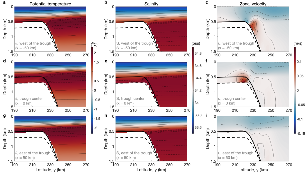
Figure 4.4: Cross-sections of potential temperature, salinity, and zonal velocity. a-c, West of the trough at x = -50 km. d-f, Trough center at x = 0 km. g-i, East of the trough at x = 50 km. The shallowest and deepest bathymetric contours are indicated by the thick solid and dashed lines, respectively.
