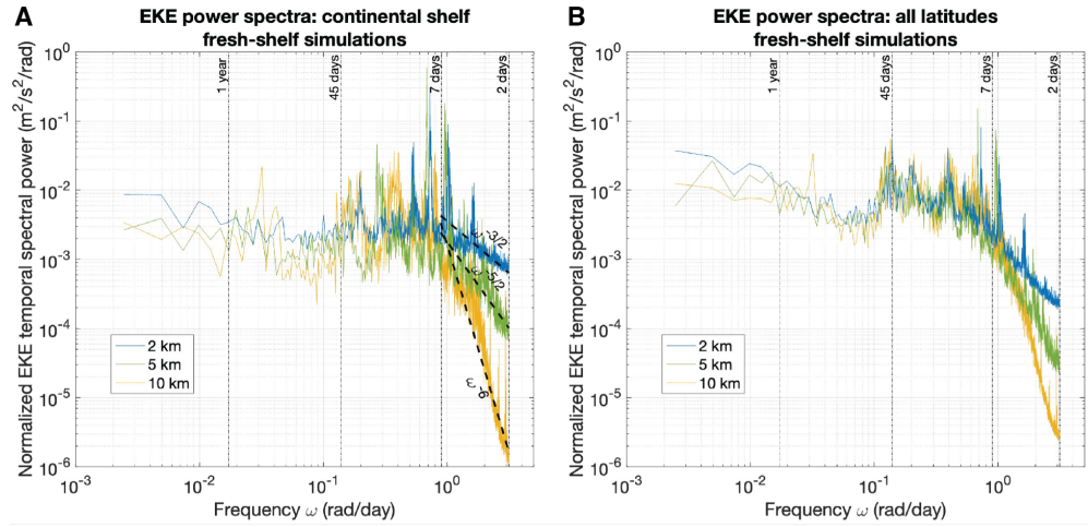
Figure 3.25: EKE power spectra for fresh-shelf simulations with different horizontal resolutions, normalized by the length of the timeseries. (A) EKE spectrum over the continental shelves (latitude y=20-125 km and depth z=0-500 m). (B) Surface 500 m EKE spectrum for all latitudes (latitude y=20-430 km excluding the 20km sponge layers at the southern and northern boundaries, and depth z=0-500 m).
