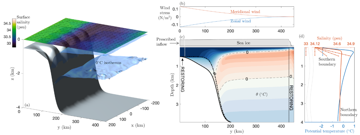
Figure 2.2: Illustration of the MITgcm Antarctic Slope Front process model (MITgcm_ASF) setup. (a) Model bathymetry, snapshot of sea surface salinity (colors), surface ocean currents (arrows), and 0^{\circ}\text{C} isotherms. (b) The steady along- and across-slope wind forcing used in the reference simulation. (c) Time- and zonal-mean sea ice thickness (the gray box, which is exaggerated) and potential temperature (the contour plot, plotted at intervals of 0.13^{\circ}\text{C} ) in the reference simulation. The thick dashed and solid black curves show the shallowest and deepest of the bathymetric contours, respectively. At the southern and northern boundaries, temperature and salinity are restored to the reference profiles across sponge layers of 20 km width. (d) The relaxation salinity (orange) and temperature (blue) profiles of the sponge layers. The northern boundary restoring (solid lines) is based on hydrography taken from the sections across the Antarctic Slope Front at Kapp Norvegia (Hattermann, 2018). The southern boundary restoring temperature and salinity are denoted by the dashed lines.
