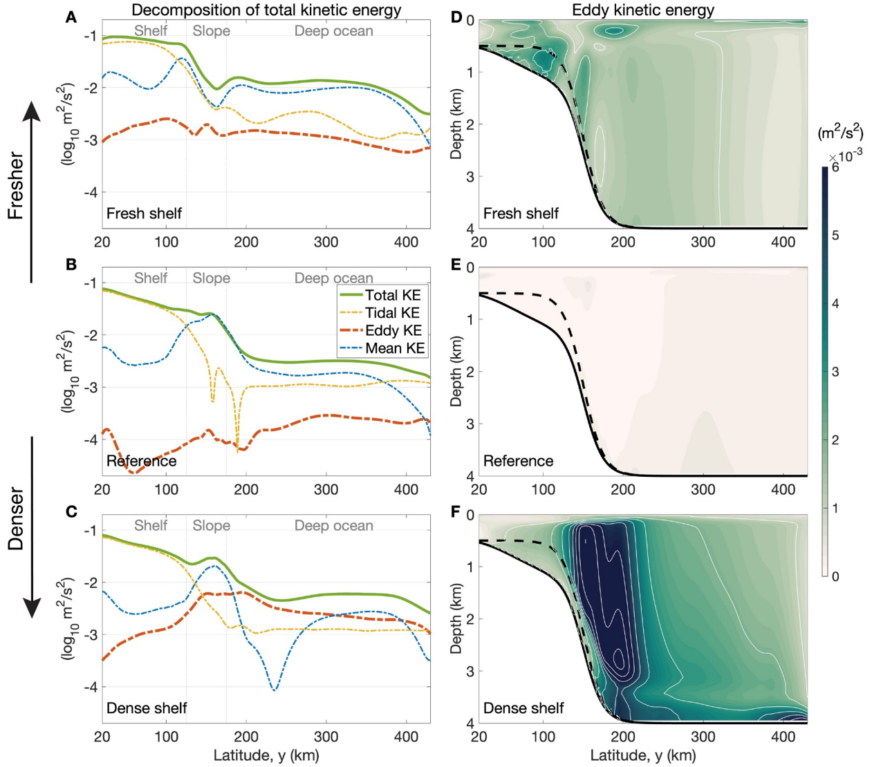
Figure 3.11: Temporal decomposition of the total kinetic energy for simulations with 2-km horizontal resolution. (A-C) Time-mean total kinetic energy, and its tidal, eddy, and mean components in the fresh-shelf, reference, and dense-shelf cases, averaged over the zonal/vertical plane. (D-F) Time- and zonal-mean eddy kinetic energy in the three cases. The colored and solid white contours show intervals of 1.5 \times 10^{-4} \text{ m}^2 \text{ s}^{-2} and 10^{-3} \text{ m}^2 \text{ s}^{-2} , respectively. The black solid and dashed curves denote the deepest and shallowest bathymetry at each latitude, respectively. The 20-km sponge layers at the northern and southern boundaries are not shown. Note the total kinetic energy and mean kinetic energy remain the same order of magnitude across simulations, while the eddy kinetic energy increases by 1~2 orders of magnitude in the fresh- and dense-shelf cases.
