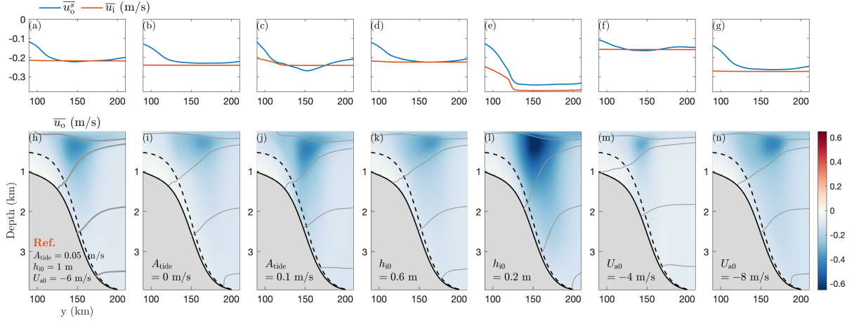
Figure 2.4: Time- and zonal-mean zonal velocity for the reference simulation (a, h), simulations with varying tidal current amplitudes (b, c, i, j), thinner sea ice at the southern boundary (d, e, k, l), and varying zonal wind speeds (f, g, m, n). The corresponding upper panels show the time- and zonal-mean zonal ice and surface ocean velocities. The gray contours denote the time- and zonal-mean neutral densities 1027.60, 1028.03, 1028.27, and 1028.35 \text{kg/m}^3 . Dashed and solid thick black curves denote the shallowest and deepest of the bathymetric contours, respectively. In these simulations, the southern boundary temperature and salinity are set to be vertically uniform ( -1.87^\circ\text{C} , 34.17 psu).
