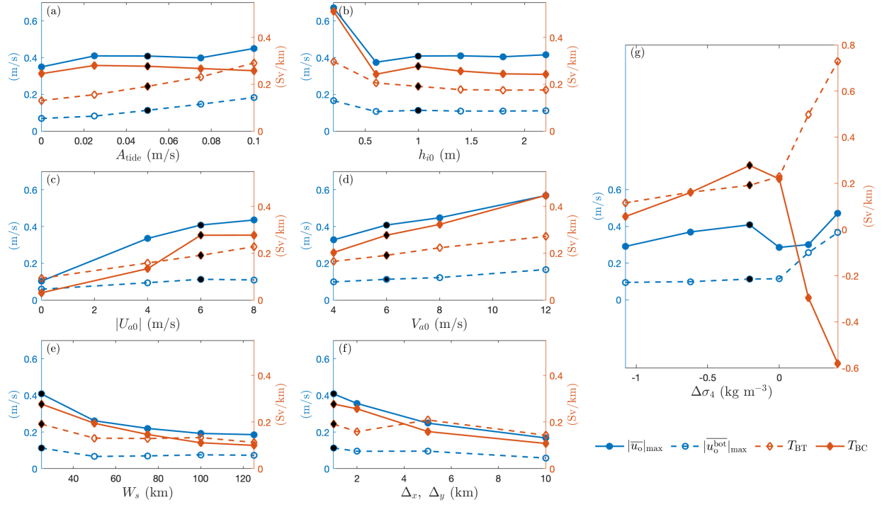
Figure 2.6: The maximum westward ocean speed |\overline{u}_o|_{\max} , maximum westward ocean bottom speed |\overline{u}_o^{\text{bot}}|_{\max} , barotropic transport T_{\text{BT}} and baroclinic transport T_{\text{BC}} per unit width over the continental slope for simulations with varying tidal current amplitude (a), sea ice thickness at the southern boundary (b), maximum westward wind speed (c), maximum northward wind speed (d), continental slope half-width (e), horizontal grid spacing (f), and ocean bottom potential density difference between the northern and the southern boundaries (g). Black dots denote the reference simulation.
