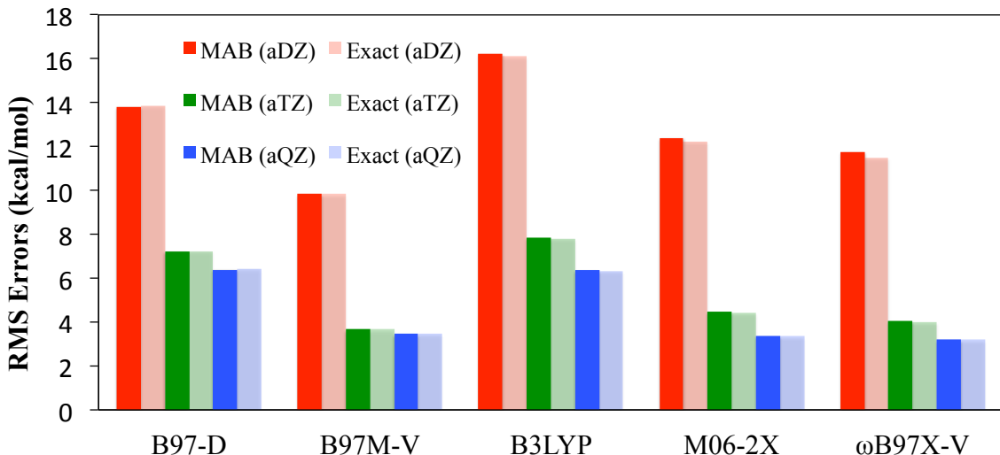
FIG. 5. Basis set convergence of the functional RMSDs for the G2 set evaluated by MAB-based methods (solid) and conventional SCF (transparent). The reference values are taken from Ref. 36. Dunning’s augmented correlation-consistent basis sets are utilized to approach the CBS limit (D: red, T: green, Q: blue). PT2 and DFPC correction schemes are applied on top of the MAB-SCF results of local (B97-D, B97M-V) and hybrid (B3LYP, M06-2X, \omega B97X-V) functionals, respectively.
