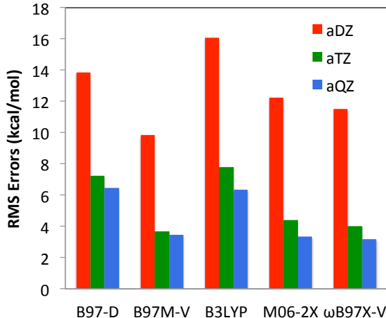
FIG. 1. Basis set dependence of the root-mean-square(RMS) errors for G2 atomization energies against the reference values from Ref. 36. Data for five functionals are collected: B97-D (GGA), B97M-V (meta-GGA), B3LYP (GH), M06-2X (GH) 39 , and \omega B97X-V (RSH). Dunning’s augmented correlation-consistent basis sets (D, T, Q) are used to systematically approach the CBS limit.
