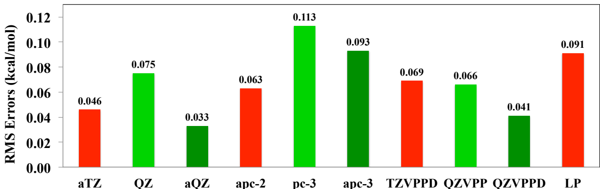
FIG. 4. Assessment of the performance of MAB+PT2 with 10 secondary basis sets. RMSDs (vs. exact SCF) for the G2 set calculated with the B97M-V functional are reported. Different colors are used to indicate distinct basis set categories: augmented triple- \zeta (red), unaugmented quadruple- \zeta (light green), and augmented quadruple- \zeta (dark green).
