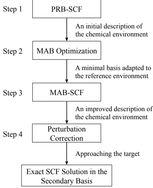
FIG. 2. Illustration of the overall MAB-SCF (PC) procedure, which includes four steps in total.
