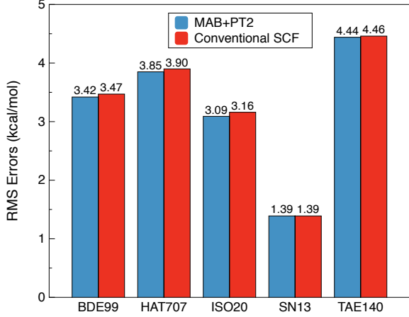
FIG. 6. B97M-V’s RMSDs for W4-11 (vs. reference values) evaluated by MAB+PT2 (blue) and conventional SCF (red). Very similar accuracy is obtained by these two SCF schemes at the B97M-V/aQZ level of theory.
