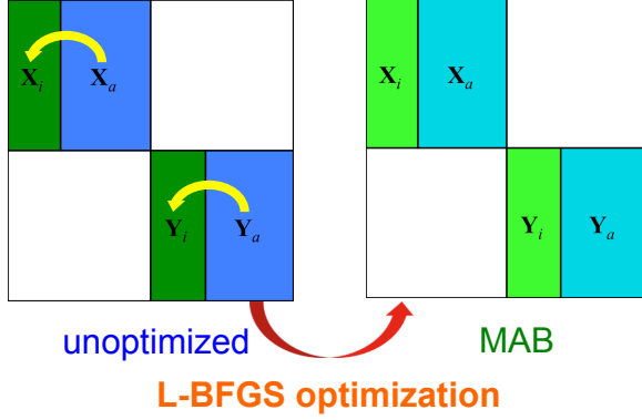
FIG. 3. Illustration of the MAB optimization procedure. Atom centers X and Y correspond to two distinct diagonal blocks of the \mathbf{B} matrix. X_i , Y_i represent the MAB functions on these sites, and X_a , Y_a represent the excluded basis functions.
