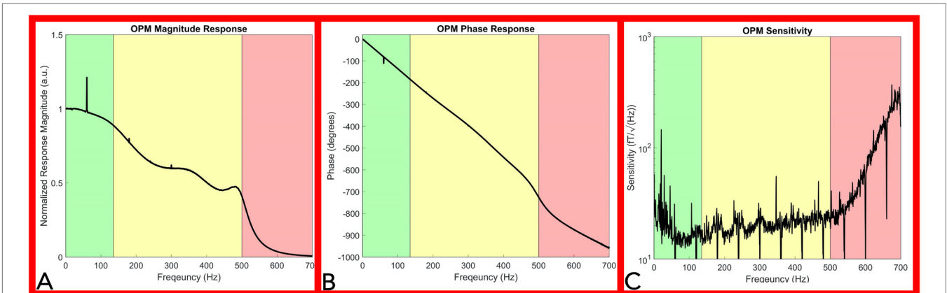
FIGURE 4 | OPM frequency response and sensitivity characterization. Panel (A): Magnitude Response of the OPM. The OPM magnitude response decreased minimally up to 135Hz (green shaded area). A moderate reduction in response was recorded up to 500Hz (yellow shaded area). Above 500Hz, a large reduction in response is noted as a direct effect of the Gen2 OPM hardware digital filter in the electronic module (red shaded area). Panel (B): Phase response of the OPM. OPM Phase response is approximately linear up to 500Hz (green and yellow shaded area). Panel (C): Sensitivity response of the OPM. OPM sensitivity was divided into three segments: below 135Hz (green shaded area), from 135 to 500Hz (yellow shaded area), and from 500 to 700Hz (red shaded area). A rapid decrease in sensitivity is noted above 500Hz. (OPM, Optically pumped magnetometer, Hz, Hertz, and fT, femtoTesla).
