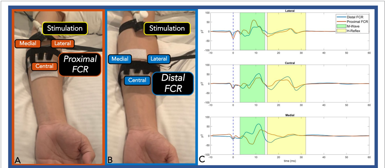
FIGURE 3 | Panel (A,B): Three OPMs were transversely placed at an equipotential level on the proximal FCR (A) and distal FCR (B). Panel (C): The centrally placed OPM (directly over the FCR) exhibited the largest H-Reflex pk-pk amplitude compared with the two radially placed OPM sensors. At the proximal FCR, the lateral and the medial OPM showed reverse polarity. At the distal FCR, where the muscle spindle is thinner, the medial OPM only detected M-Wave activity. The M-wave and the H-Reflex responses are highlighted green and yellow, respectively. (OPM, Optically pumped magnetometers, FCR, Flexor carpi radialis, pT, picoTesla, and ms, milliseconds).
