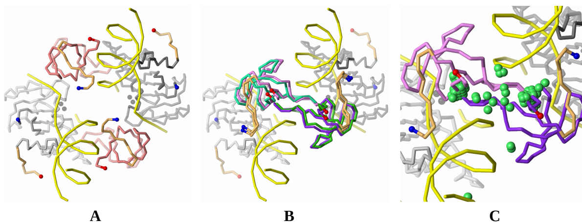
Figure 2: The PFV CTD docks between the two active sites. (A) Each crystallographic CTD (red tubes) contacts both vDNA molecules (yellow tubes), but the active-site region between the two 3'-ends of the cleaved vDNA strands is unoccupied. The CCDs (gray with spheres representing the Mn ions) and the CTDs have attached L2 residues (orange) that were included in the docking calculations. N- and C-termini are shown as blue and red spheres. (B) Two symmetry-related pairs of docked CTD placements (ranks 2 and 12, green and ranks 4 and 15, purple) represent the two clusters making up 29/30 of the top-ranked positions. The docked CTDs occupy the central active-site region between the two vDNA molecules, reducing the distance between the CCD C-terminus and the CTD N-terminus by 12 Å. (C) The 100 top-ranked docked CTD positions, represented by their geometric centers (green spheres), are concentrated in the region over the two active sites. Of these, 78 had an RMSD within 5 Å of the symmetry-related pair (purple).
