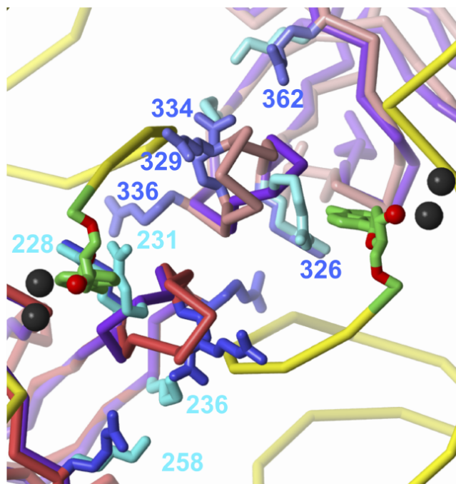
Figure 3: CTD loop 326-337 fills the region between the two PFV-IN active sites. The view is looking down on the host-DNA-binding face of the IN assembly. The loops of the two docked CTDs (red, lower left and light red, upper right) put eight Arg residues (dark blue side chains and labels) between the two 3'-nucleotides (green with red oxygen atoms) of the vDNA (yellow) bound at the active sites (indicated by Mn ions, black spheres). The corresponding loops of the HIV CTD (purple) position four Arg and two Lys residues (light blue side chains and labels) in the same area. PFV CTD Arg 362, which corresponds to HIV CTD Lys 258, may also contribute to vDNA binding near the active site.
