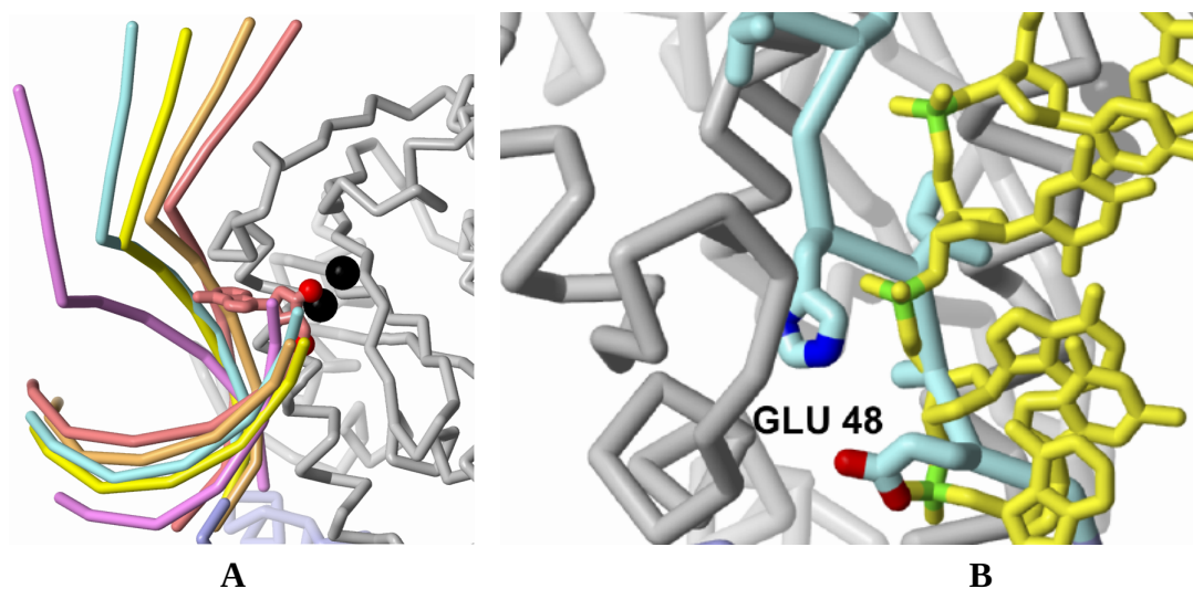
Figure 4: The L1 of HIV-IN NTD-CCD structure clashes with bound vDNA. (A) Docking vDNA to the HIV NTD+CCD. In the absence of the L1 linker, the vDNA fits well at the CCD active site (gray tubes with two active-site Mn ions as black spheres), but shows a wide range for the 2-nucleotide overhang (upper left). Docked vDNA are rank 14 (red, RMSD = 2 Å), rank 1 (orange, RMSD = 3.9 Å) rank 2 (yellow, RMSD = 6.0 Å) rank 13 (light blue, RMSD = 8.6 Å) and rank 14 (purple, RMSD = 11.7 Å). (B) The HIV L1 (light blue) blocks the vDNA-binding site on CCD. L1 residues Glu 48, Ala 49, and Ile 50 occupy the groove that binds the phosphate backbone of the uncleaved vDNA strand (yellow). The Glu 48 side chain lies in a pocket occupied by a phosphate group (green P atom).
