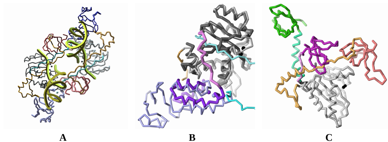
Figure 1: Variations in integrase structures. (A) The two inner subunits of the PFV-IN assembly (PDB ID 3OY9), 30 looking down on the vDNA-binding face. Host DNA binds on the opposite face. The two protein chains (upper with thin tubes, lower with thicker tubes and paler colors) are colored blue - NTD, light blue - L1, gray - CCD, orange - L2, and red - CTD. The L1 and L2 linker regions extend over the region between the two active sites and contact the vDNA (yellow ribbons). The active-site Mn ions (black spheres) and NTD Zn ion (light blue spheres) are also shown. (B) The L1 linkers in HIV-IN and PFV-IN have very different positions. In the HIV NTD-CCD structure 3F9K, 16 L1 (pink) lies in a groove on the surface of the CCD (dark gray) and connects to the adjacent NTD (purple), creating a compact structure. In PFV-IN (thin tubes), the CCD (gray) and its contacting NTD (lavender) are attached to different protein chains and L1 (light blue) extends through solvent (as shown in (A)) so that the NTD and CCD in the same protein chain do not contact each other. A second HIV NTD-CCD structure 15 (PDB ID 1K6Y, not shown) has no density for L1 and the NTD was assigned to a very different position than in 3F9K. Subsequent analysis 5 revealed that the crystal lattice includes an NTD that matches the NTD position in 3F9K. (C) Differences in the CTD position among integrases. Superposition of the CCDs (gray, shown for PFV-IN only) shows the dramatic variation in L2 conformation and CTD position among PFV-IN (orange and red), HIV-IN (light green and green, PDB code 1EX4), 17 and ASV-IN (pink and magenta, PDB code 1C0M). 18 Further variation is found in the second subunit of the HIV-IN and ASV-IN CCD-CTD structures, and in SIV-IN, 33 which has a helical L2 of the same length as HIV-IN.
