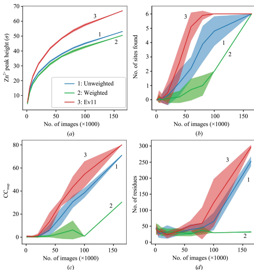
Figure 5 Effect of image count on autobuilding success. For each of the three protocols, increasing numbers of images were processed. The anomalous peak height for the Zn 2+ atom (a), the number of heavy-atom sites found (out of six) (b), the known model-to-map CC (c) and the number of residues built (d) are shown versus the number of images in the data set. In each case, shaded areas indicate the standard deviation of either the ten subsamples (data sets 1000–100 000) or the ten random seeds (full data set, 164 063 images). Note that for (b) certain data points have the same number of sites found in all trials and hence have no standard deviation.
