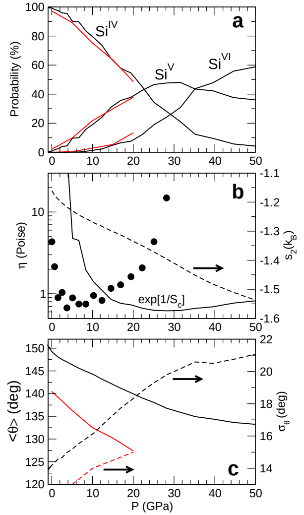
Figure 8: (Color online) a) Fraction of 4-, 5- and 6-fold silicon atoms as a function of pressure in the NS2 (black curves) and MORB liquid (red curves). b) Simulated viscosity of the NS2 liquid at T=2000 K (filled black circles, same as Fig. 3), compared to an Adam-Gibbs viscosity computed from a structure-related configurational entropy S_c . Right axis: Entropy s_2 (broken line) computed from equ. (8). c) Mean angle around the bridging oxygen (BO) atom and corresponding second moment (standard deviation) of the bond angle distribution (right axis).
