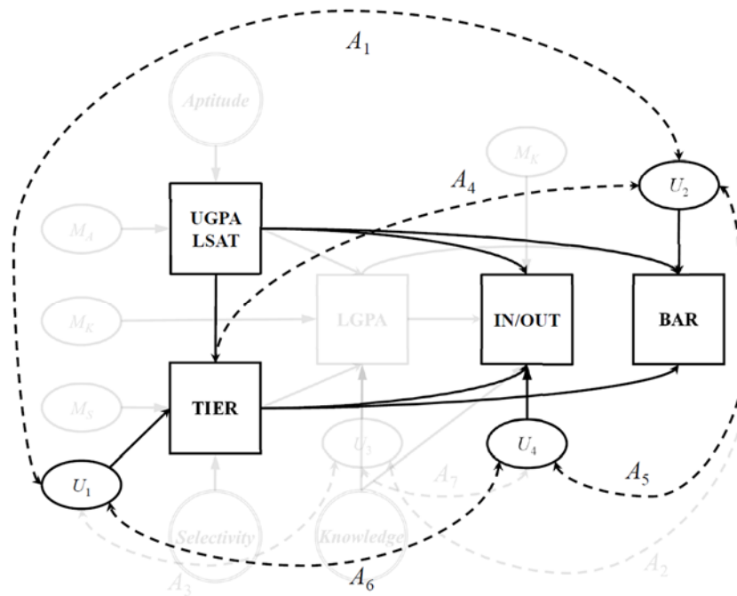
Figure 5: Sander's Causal Model
