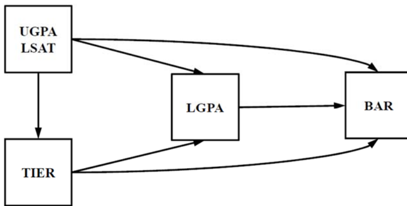
Figure 2: Sander's Causal Model (Manifest Indicators)
