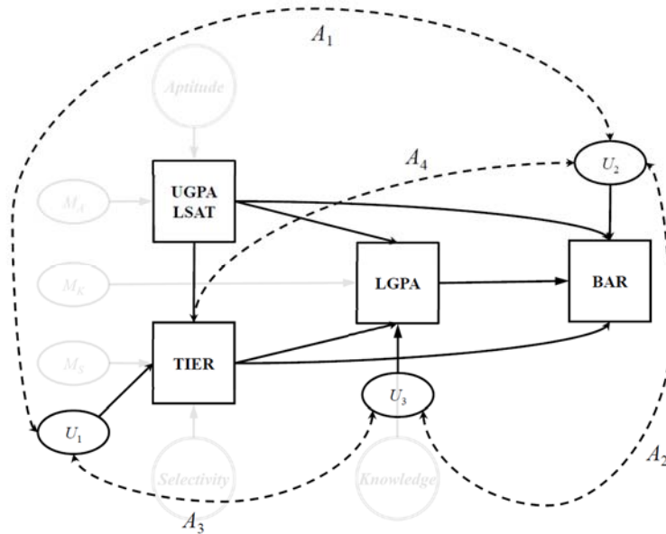
Figure 4: Sander's Causal Model
