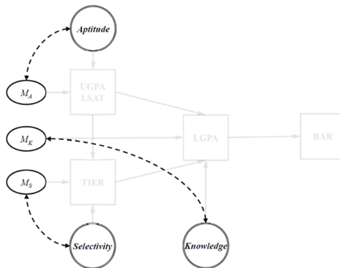
Figure 17: Sander's Causal Model (Condition 1 Measurement Errors)
