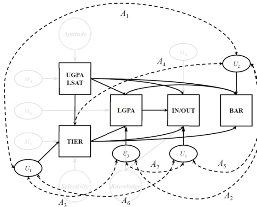
Figure 6: Sander's Causal Model
