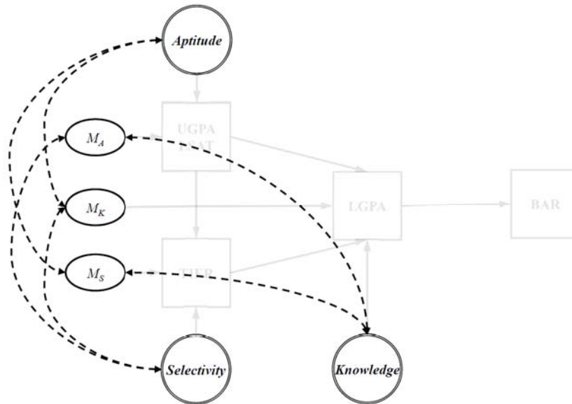
Figure 19: Sander's Causal Model (Condition 2 Measurement Errors)
