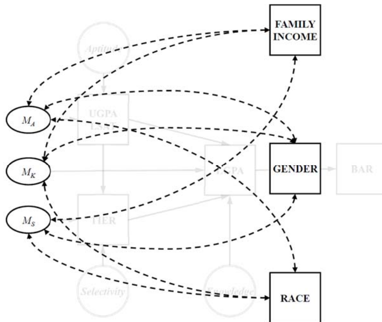
Figure 19: Sander's Causal Model (Condition 2 Measurement Errors)
