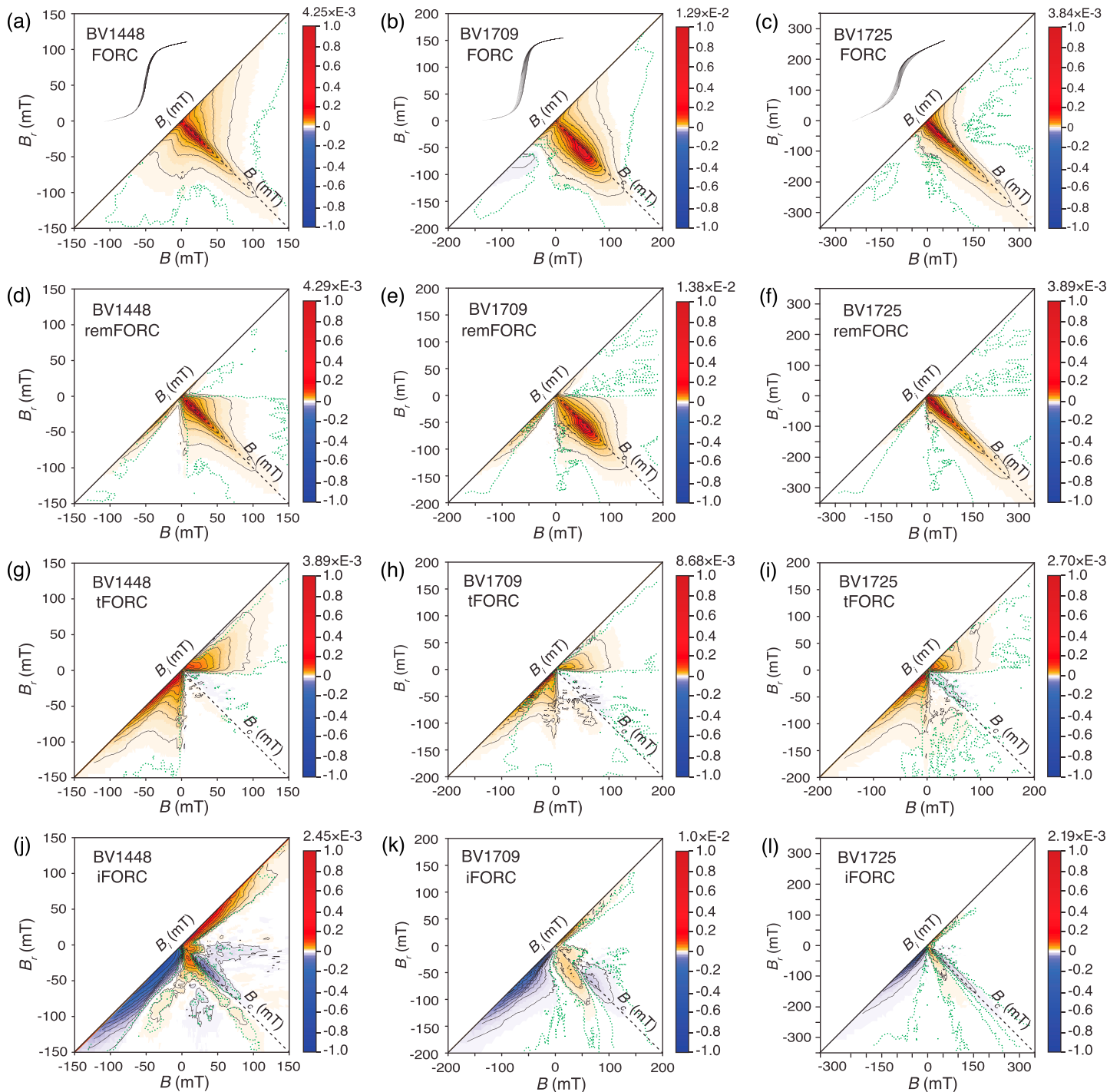
Figure 9. Domain state diagnosis for the Butte Valley sediment core (Roberts et al., 1996) using the FORC-type measurements of Zhao et al. (2017). From top to bottom, conventional FORC, remFORC, tFORC, and iFORC diagrams for samples for which conventional FORC diagrams are shown in Figure 8: (a, d, g, and j) BV1448 (dominantly detrital vortex state magnetite), (b, e, h, and k) BV1709 (magnetostatically interacting SD greigite), and (c, f, i, and l) BV1725 (mixture of noninteracting SD and vortex state magnetite and higher-coercivity hematite). See text for discussion. Dashed green contour lines represent the 0.05 significance level determined following Heslop and Roberts (2012b). All samples were measured using an irregular measurement grid (Zhao et al., 2015) with 100-ms averaging time and were processed with SF = 5 for BV1448 and SF = 4 for BV1709 and BV1725.
