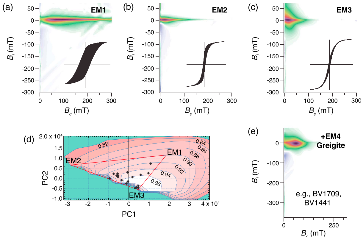
Figure 10. Illustration of FORC unmixing of conventional FORC diagrams for the Butte Valley sediment core (Roberts et al., 1996). Three EMs are identified using PCA along with a greigite EM with behavior that is distinct and isolated from that of the other three EMs. FORC diagrams for each EM are as follows (a) high-coercivity (>300 mT), weakly interacting SD hematite with small SP contribution, with mainly uniaxial anisotropy, but with hints of multiaxial anisotropy (EM1) ( M_{rs}/M_s of the extracted FORCs = 0.66, which is consistent with multiaxial anisotropy in hematite); (b) weakly interacting SD magnetite, with mainly uniaxial features (EM2), and a secondary SP/SD peak at the origin, which is responsible for the wasp-waisted extracted FORCs ( M_{rs}/M_s = 0.385 ); and (c) vortex state magnetite (EM3). (d) The mixing space is defined using two principal components, PC1 and PC2, where measured FORC data fall within a ternary mixing space with vertices represented by the three EMs in (a–c). The contours in (d) represent the zone in which FORC diagrams are physically meaningful; metrics used to define these contours were used to guide EM placement. EM2 was placed as far as possible from EM3 to remove traces of the vortex state EM3 and to isolate the pure SD EM2 signal. Placement of EM1 is flexible, and interpretation is clear regardless of its exact placement. All samples fall inside the mixing triangle, which makes identification of EM3 straightforward. (e) FORC diagram for the isolated interacting SD greigite component (EM4). VARIFORC smoothing parameters (see Egli, 2013) used in all FORC diagrams are s_{c,0} = 5 , s_{c,1} = 6 , s_{b,0} = 12 , s_{b,1} = 12 , and \lambda_c = \lambda_b = 0.1 , with a correction of 0.0013102 for a vertical offset of the central ridge in EM1 and EM2 due to magnetic viscosity caused by time asymmetry of the FORC measurement (e.g., Pike, Roberts, & Verosub, 2001).
