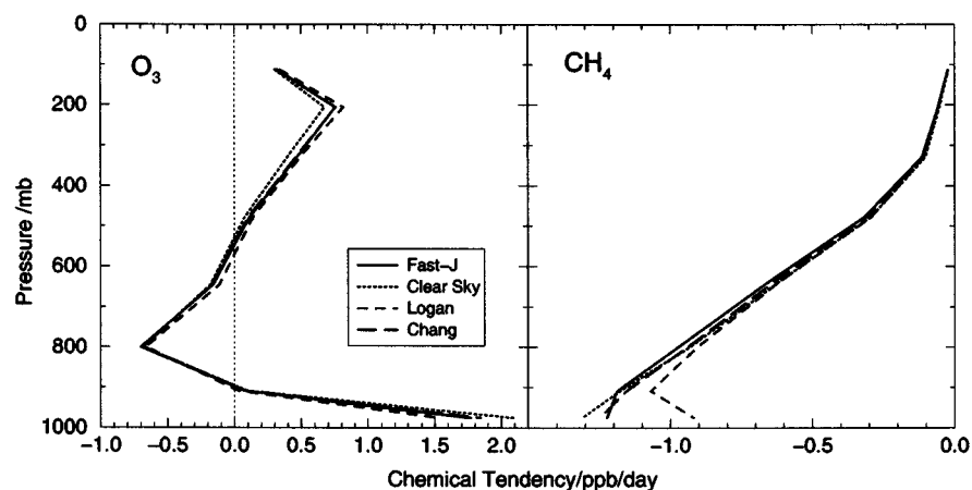
Figure 3. Net chemical tendencies (ppbv/day) of \text{O}_3 and \text{CH}_4 as a function of pressure (mb). The rates are globally averaged from the UCI CTM for the third week of September and demonstrate the impact of different treatments of photolysis: Clear-sky, Logan and Chang methods, and Fast-J.
