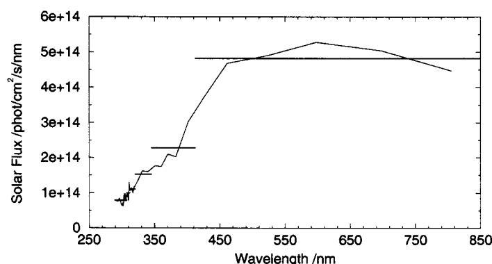
Figure 12. Top-of-atmosphere solar flux (photons \text{cm}^{-2} \text{s}^{-1} \text{nm}^{-1} ) for the 40 wavelength bins longward of 289 nm in a standard photolysis calculation (thin line) and the corresponding 7 bins for Fast-J (thick horizontal lines).
