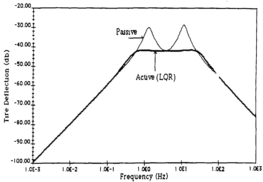
Fig.13 Active Suspension for Road Holding [15]
