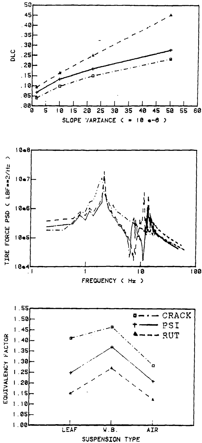
Fig.11 Effect of Suspension Type on Vehicle Response and Road Damage
