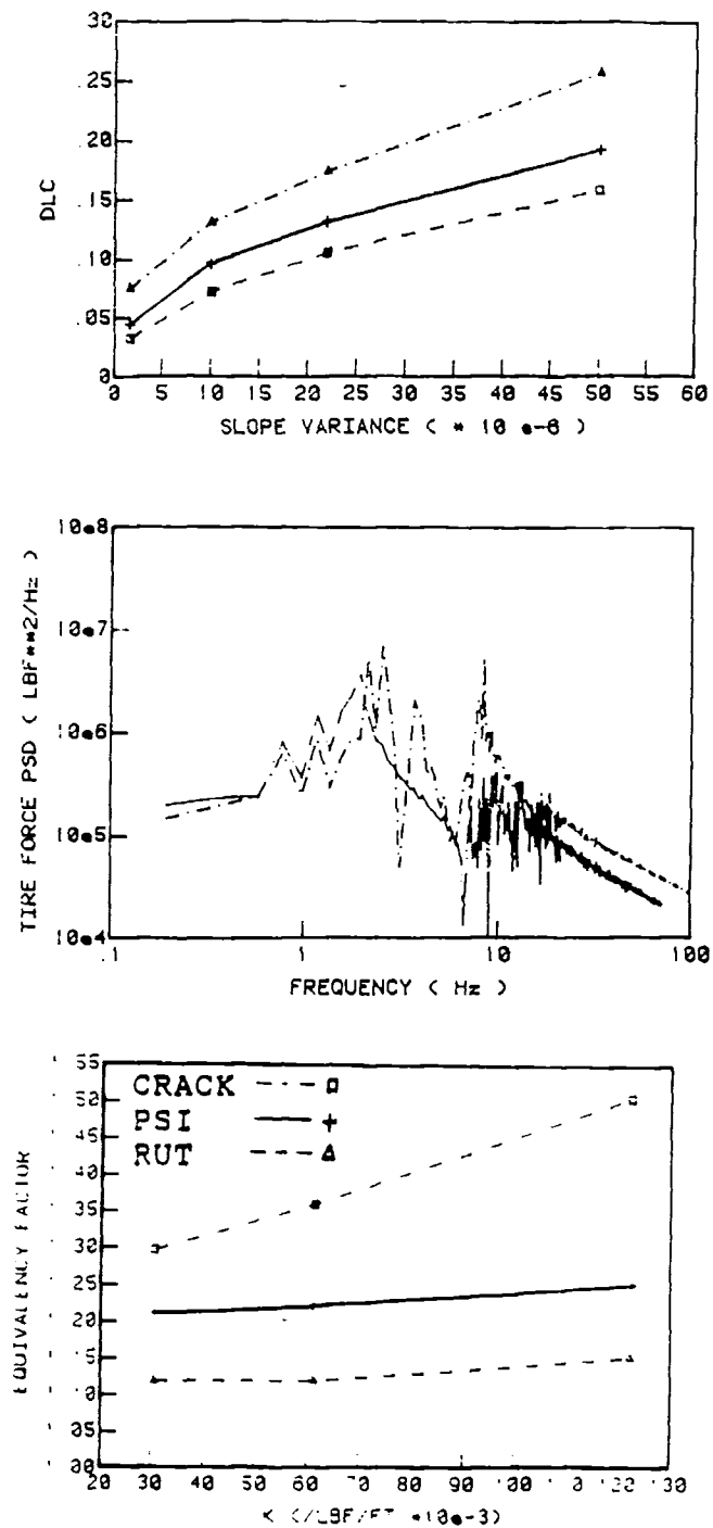
Fig.9 Effect of Spring Stiffness on Vehicle Response and Road Damage a) Leading Drive Axle DLC versus SV □ — — — K = 30,600 lbs/ft + — — — K = 61,200 lbs/ft ( standard ) △ — — — K = 122,400 lbs/ft b) Leading Drive Axle Tire Force PSD at SV = 22 \times 10^{-6} c) Effect of Leaf Spring Stiffness on Pavement Damage
