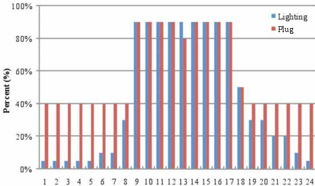
Figure 3 Initial Schedules of Lighting and Plug Power Densities on Weekdays
