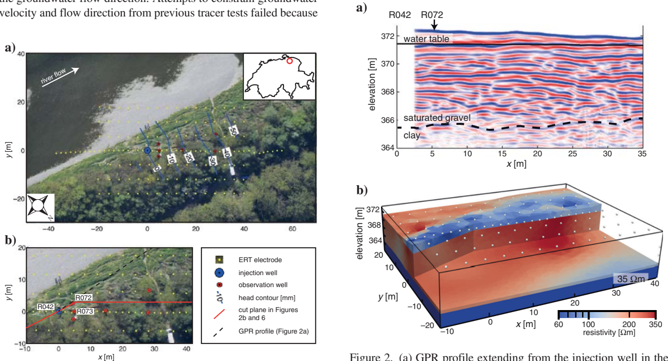
Figure 2. (a) GPR profile extending from the injection well in the direction of the initial tracer movement. The profile is extracted from the data of Doetsch et al. (2012). (b) Resistivity model obtained from ERT inversion of data acquired prior to tracer injection. This baseline model is used as the starting and reference model for the inversion. Dots at the surface are electrode positions. Resistivities in the unsaturated upper zone vary from 60 to 300 Ωm (blue to red in the model); they are expected to be a function of water and clay content of the soil. The saturated gravel aquifer with resistivities of 200–350 Ωm (uniformly red) is underlain by a clay aquitard with a resistivity of \sim 35 Ωm (dark blue).
