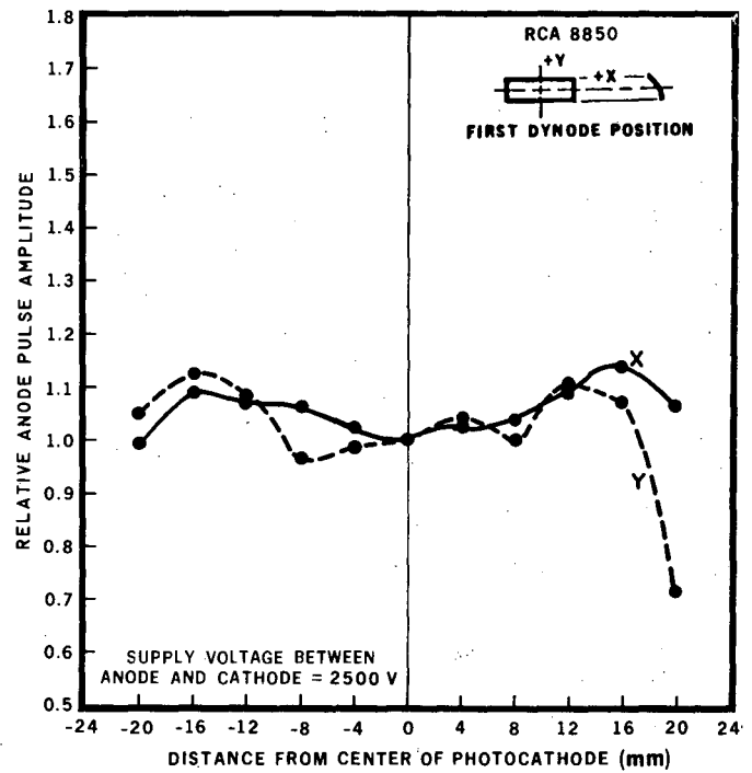
Fig. 14 - Collection and quantum efficiency uniformity as a function of the position of the photocathode sensing area, for RCA 8850 photomultiplier.
