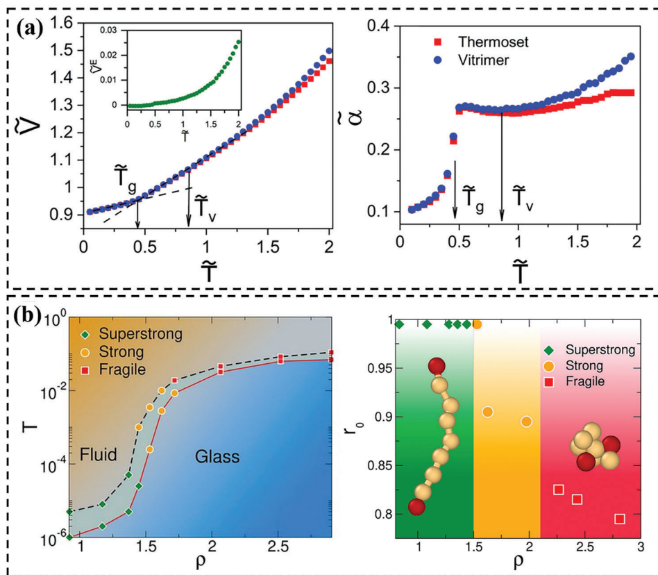
Figure 4. a) Reduced (left) specific volume and (right) thermal expansion coefficient as a function of reduced temperature \bar{T} ( \bar{T} = k_B T/\epsilon , k_B is the Boltzmann constant, \epsilon is the well depth of Lennard–Jones potential), \bar{T}_g and \bar{T}_v denote the glass transition temperature and the topology freezing temperature, respectively. Reproduced with permission. [21b] Copyright 2020, American Chemical Society. b) Simulated phase diagram as a function of temperature T and bulk density (left). Distance r_0 corresponds to the main peak of the radial distribution function g(r) as a function of vitrimer bulk density (right). Reproduced with permission. [82] Copyright 2019, PNAS.
