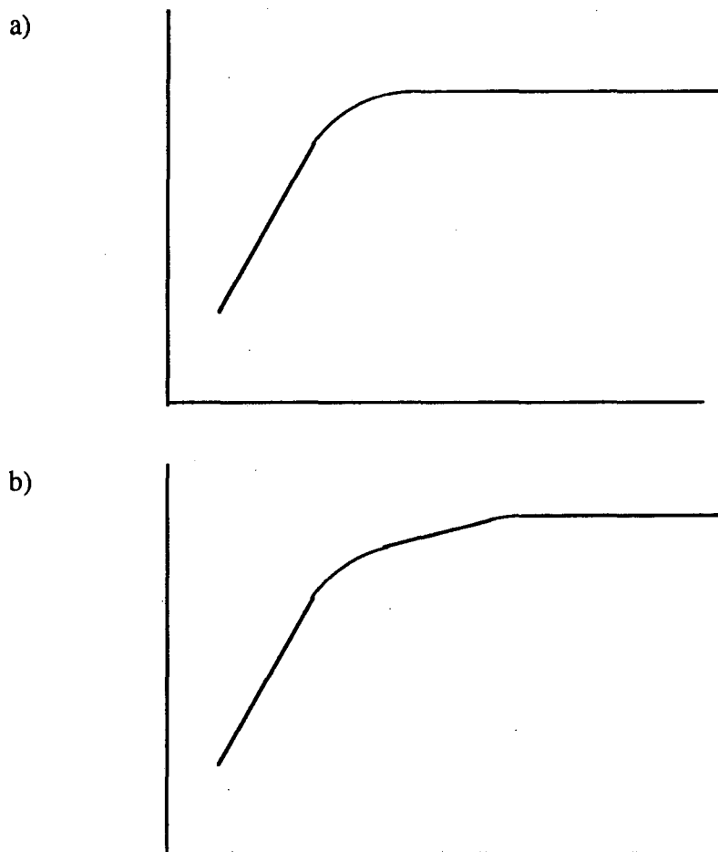
Figure 4.11. a) Expected behavior of N apparent as a function of preparation time for a collection of isolated spin clusters with uniform spin-spin coupling strength magnitude.
