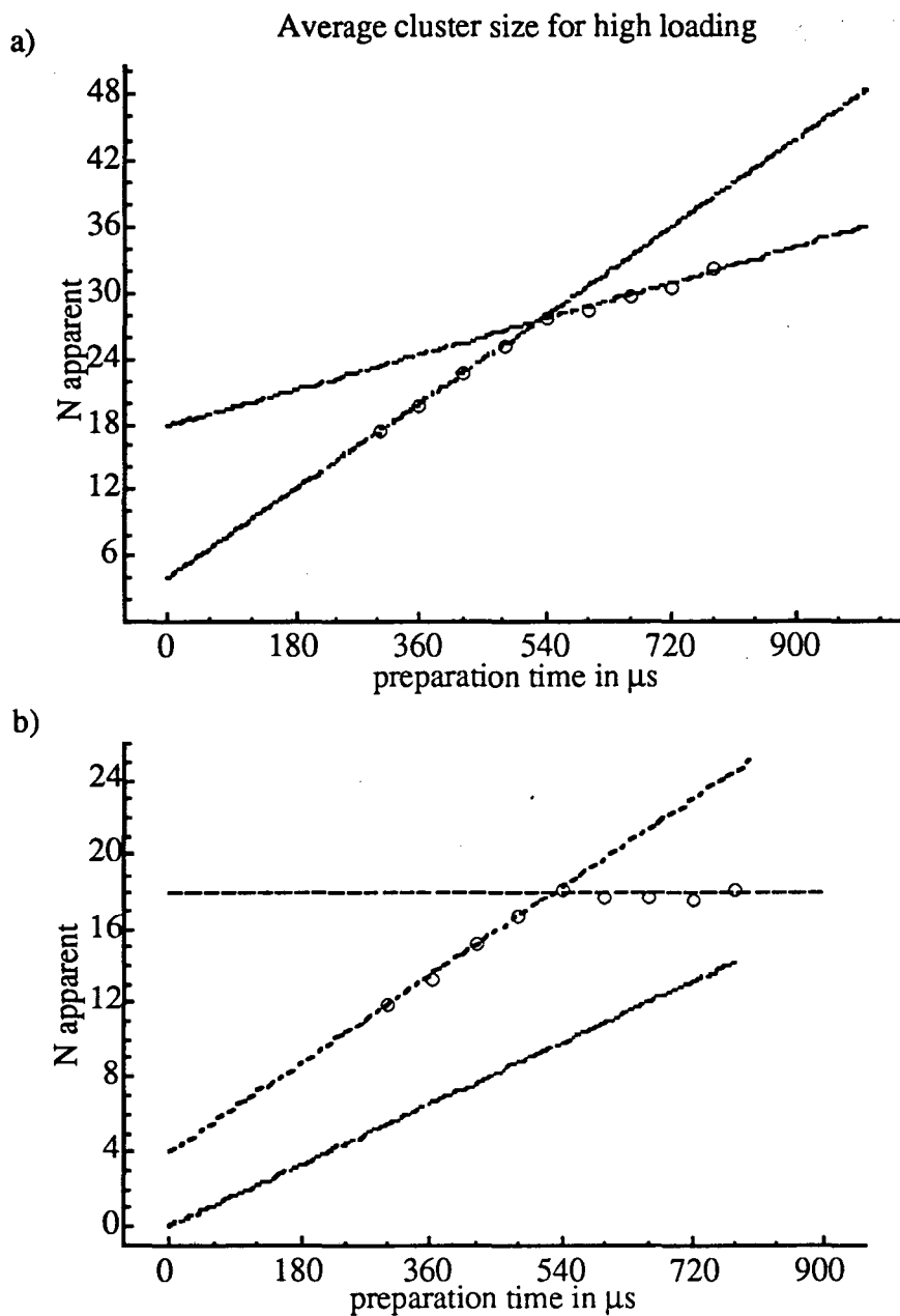
Figure 5.8. a) N apparent as a function of preparation time for NaY zeolite containing a bulk concentration of three benzene molecules per supercage. b) The difference between the data in a) and a line drawn through the origin with a slope determined by a least-squares fit of the data acquired after 500 \mu\text{s} .
