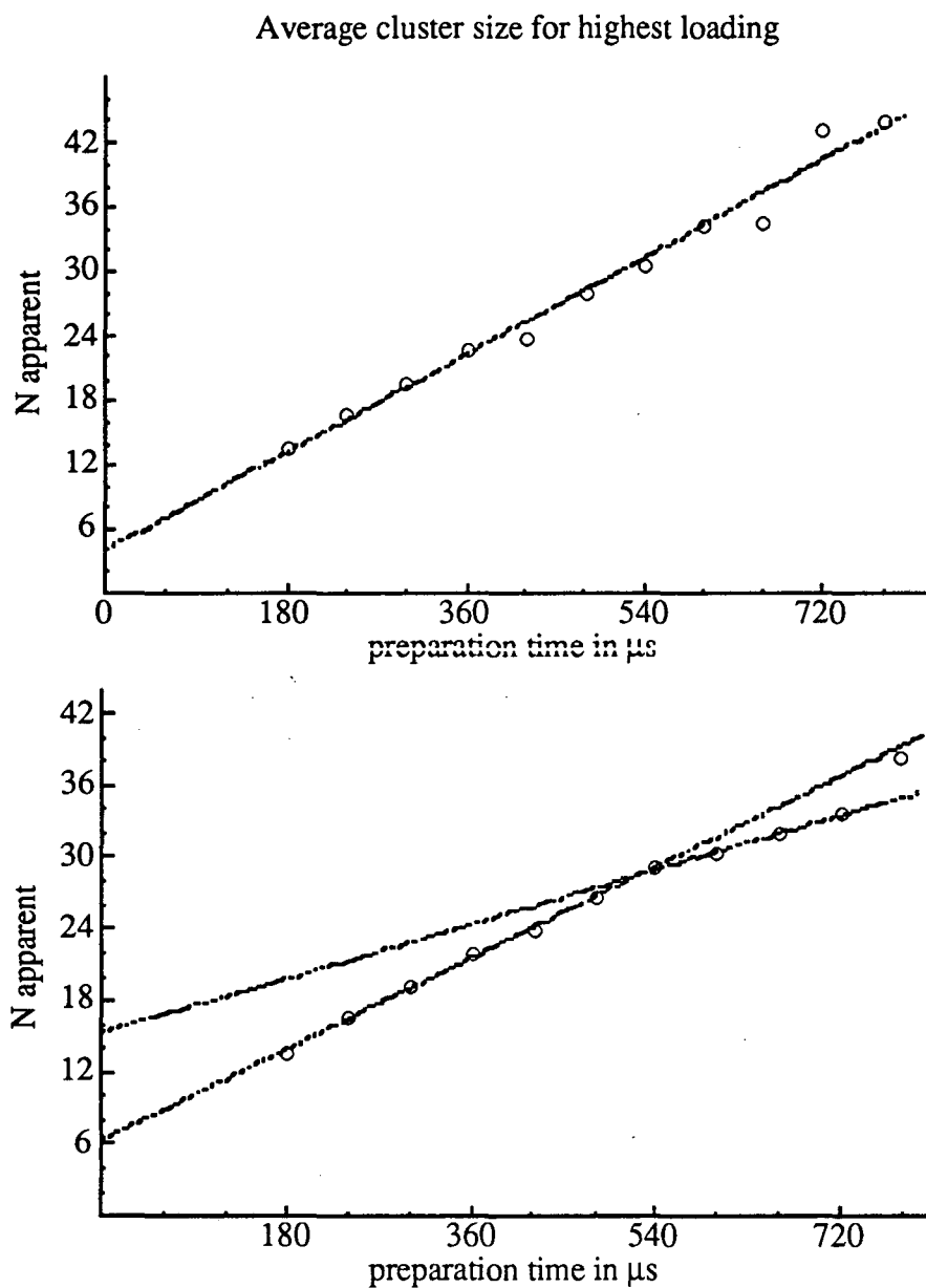
Figure 5.9. a) N apparent as a function of preparation time for NaY zeolite containing benzene at an average concentration of four molecules per supercage.
