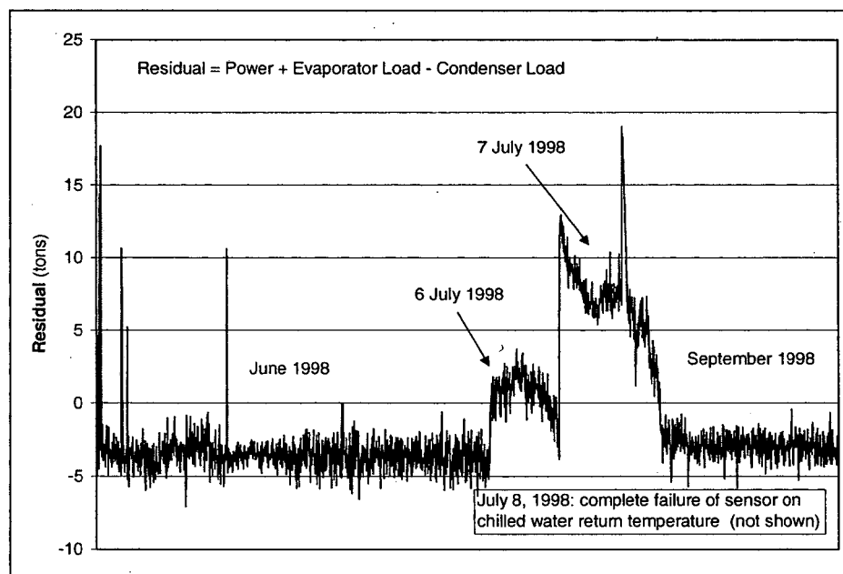
Figure 3. Energy balance residual for a period including power spikes and a sensor failure.
