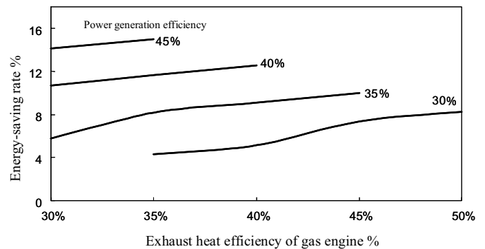
Figure 10 Gas Engine Efficiency and Energy Saving
