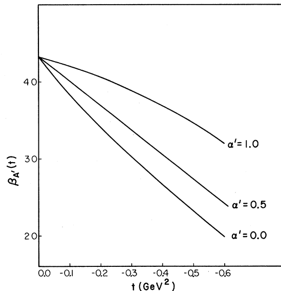
FIG. 2. \beta(t) = \text{Im } A'(\nu, t)/\nu^{1+\alpha't} for various values of \alpha' as a function of t . E_{\text{lab}} = 2.0 GeV/c.
