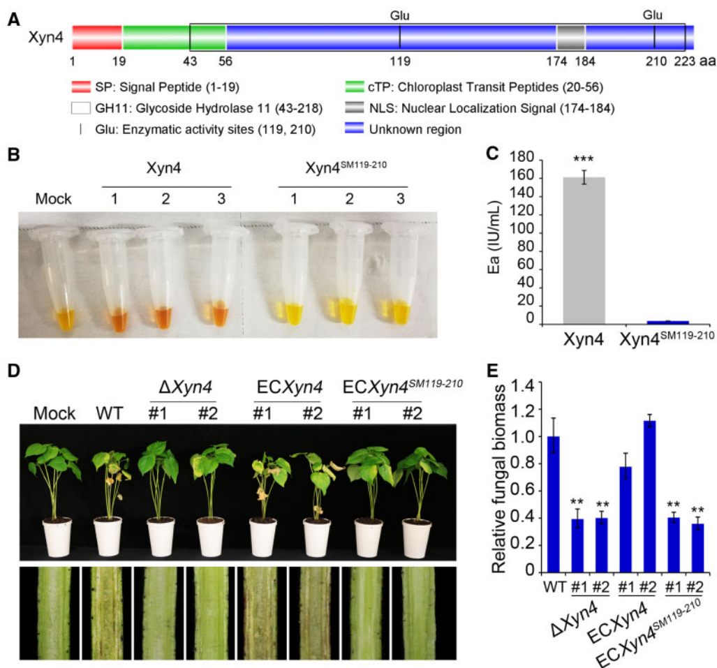
Figure 4 Function identification of enzyme activity sites of xylanase VdXyn4 from V. dahliae . A , Sequence characteristics of VdXyn4, including: SP, N-terminal cTP, Glu, two enzymatic activity sites, NLS sequence, Glycoside hydrolase 11 (GH11) domain. Numbers in schematic represent the position of the amino acid (aa) residues. B and C , Xylanase activity determination of WT and two site-directed mutants. Induction was carried out with beechwood xylan as the only carbon source in each case. Ea represents enzyme activity. Error bars represent \pm SE of the mean. Asterisks represent statistical significance at P < 0.001 based on unpaired Student's t tests. D , Phenotypes of cotton seedlings inoculated with VdXyn4 gene deletion strains and complementary transformants. The cotton seedlings were inoculated with sterile water (Mock), WT V. dahliae , VdXyn4 gene deletion strains, and complementary transformants. The disease symptoms are shown at the top and the discoloration of the shoot longitudinal sections is shown at the bottom at 3 wpi. E , The fungal biomass of the gene deletion strains and corresponding ectopic transformants on cotton were determined by quantitative PCR. The V. dahliae elongation factor 1- \alpha ( EF-1 \alpha ) was used to quantify fungal colonization, and the cotton 18S served as an endogenous plant control. EC represents ectopic complement transformants. Error bars represent \pm SE of the mean. Asterisks represent statistical significance at P < 0.01 based on unpaired Student's t tests.
