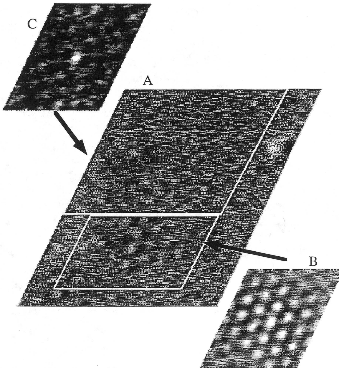
Figure 9.5 Image of Diffusing Sulfur and Partial Correlation Images An STM image (A) of a sulfur island surrounded by an area of diffusing sulfur. In the correlation image (B) of the island area all the peak heights are roughly equal. However, in the correlation image (C) of the diffusing atoms, the center peak is much higher than the surrounding peaks because the coverage in this area is low.
