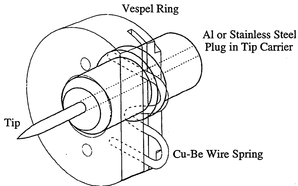
Figure 3.4 Drawing of the Tip Attachment
