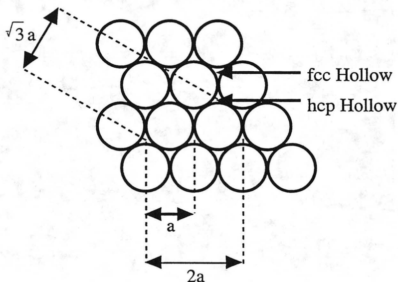
Figure 9.2 Distances Between High Symmetry Points on Re(0001)
