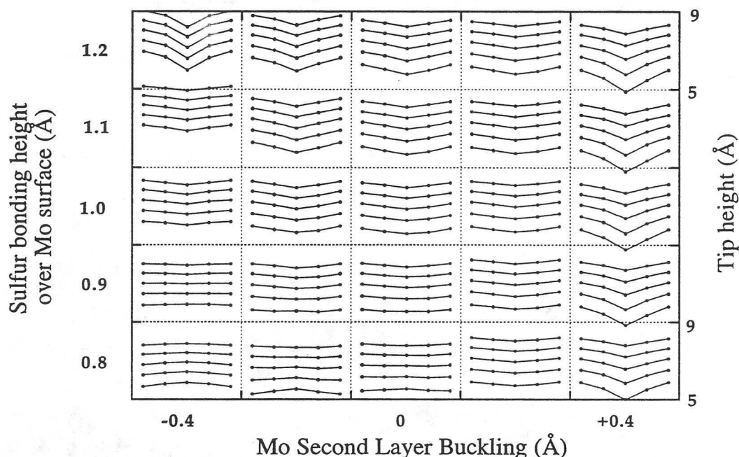
Figure 8.4 Theoretical Image Shape vs. Surface Structure (Pt tip)
