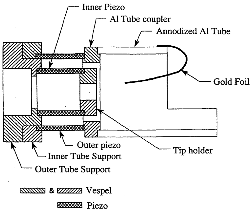
Figure 3.3 Drawing of the STM Head
