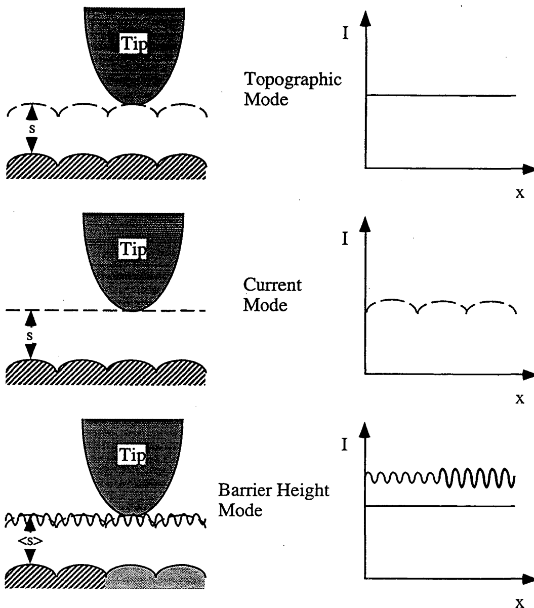
Figure 2.5 STM Imaging Modes
