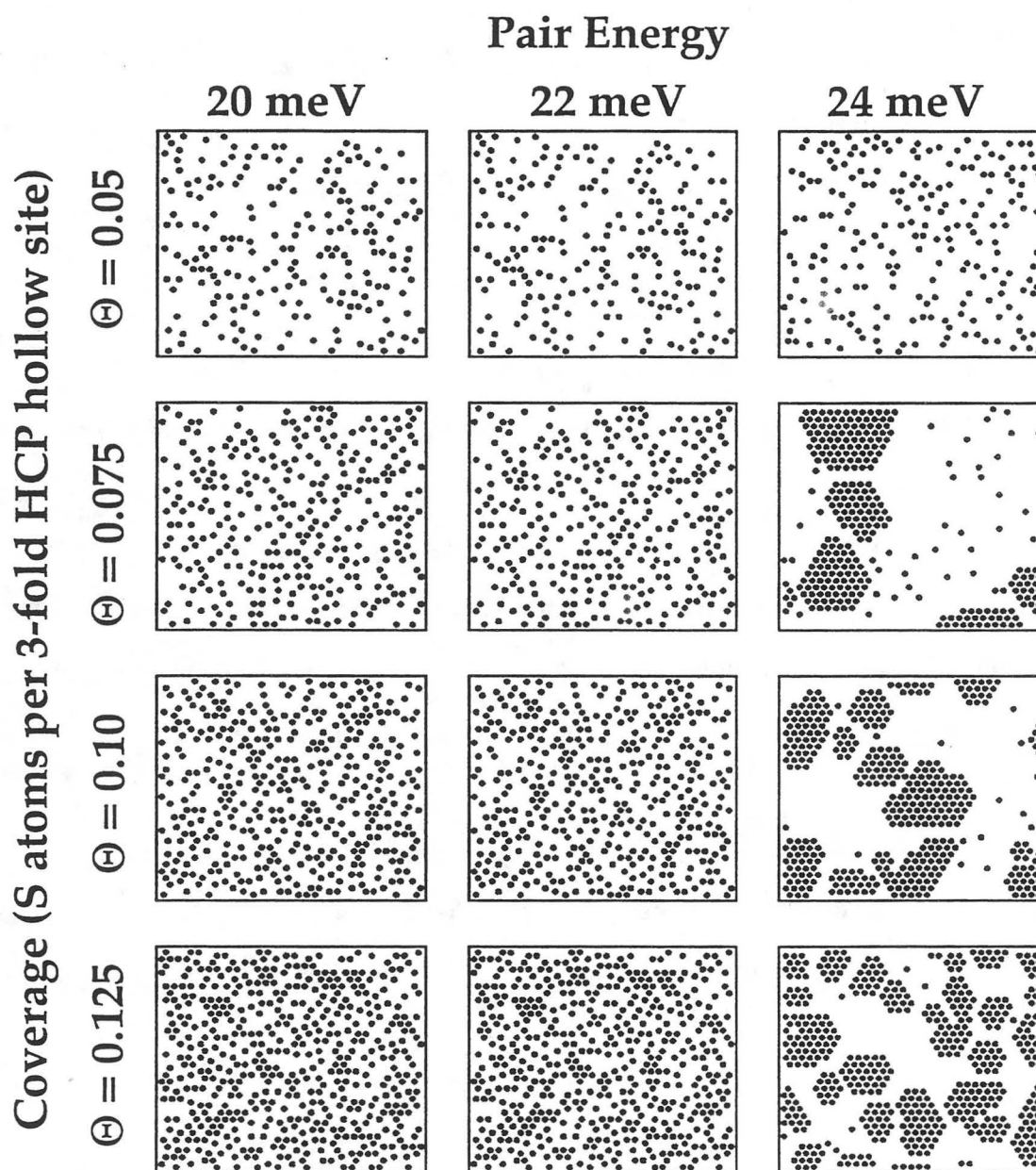
Figure 9.9 Phase Transition
