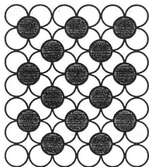
Figure 7.3 A Model of the Hollow Site c(2 \times 2) Overlayer
