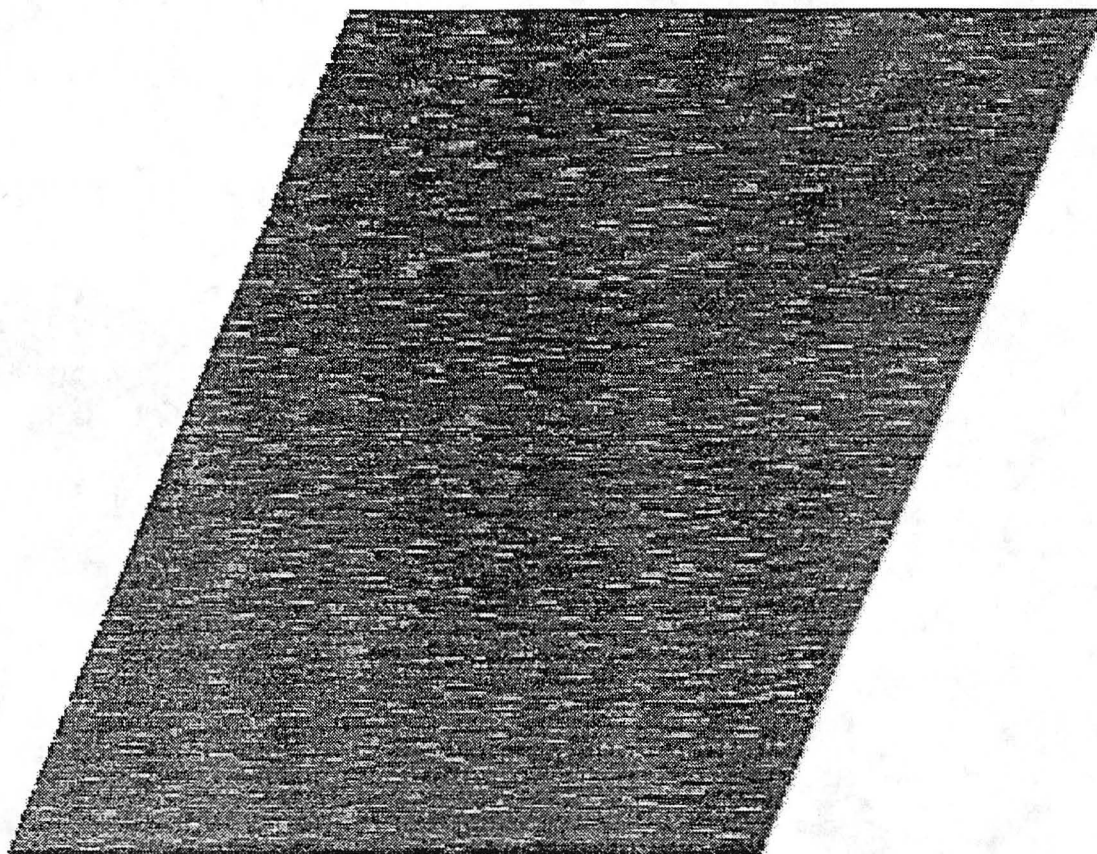
A. Raw STM Image
