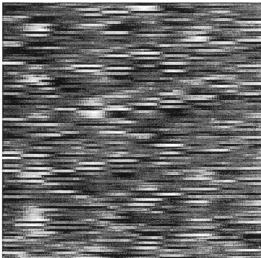
Figure 9.3 Magnified Raw Data Image of Diffusing Sulfur
