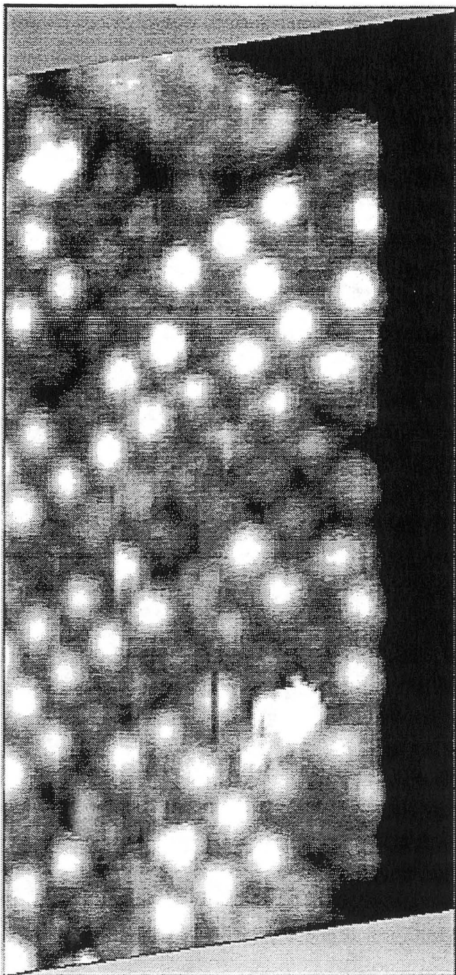
Figure 11.1 STM Images Of Gold On The Mo(100) Surface
