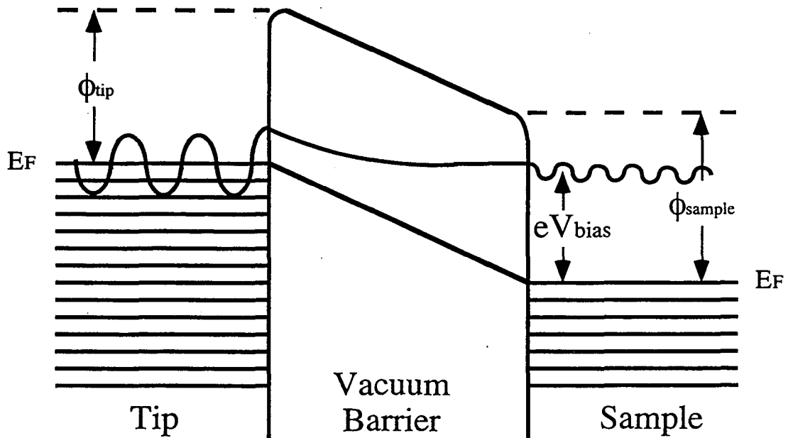
Figure 2.1 A Model Of The Tunneling Barrier
