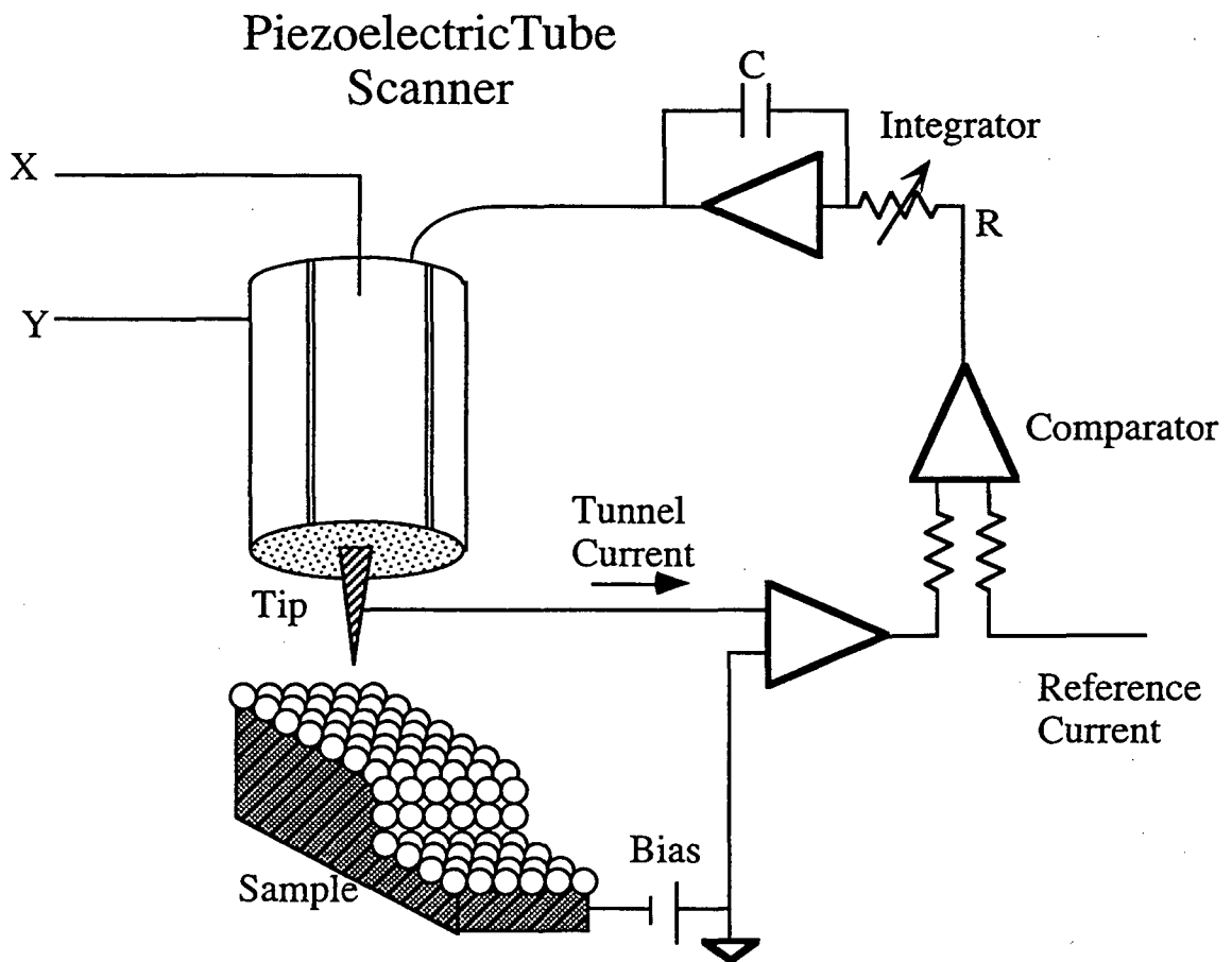
Figure 2.4 STM Model
