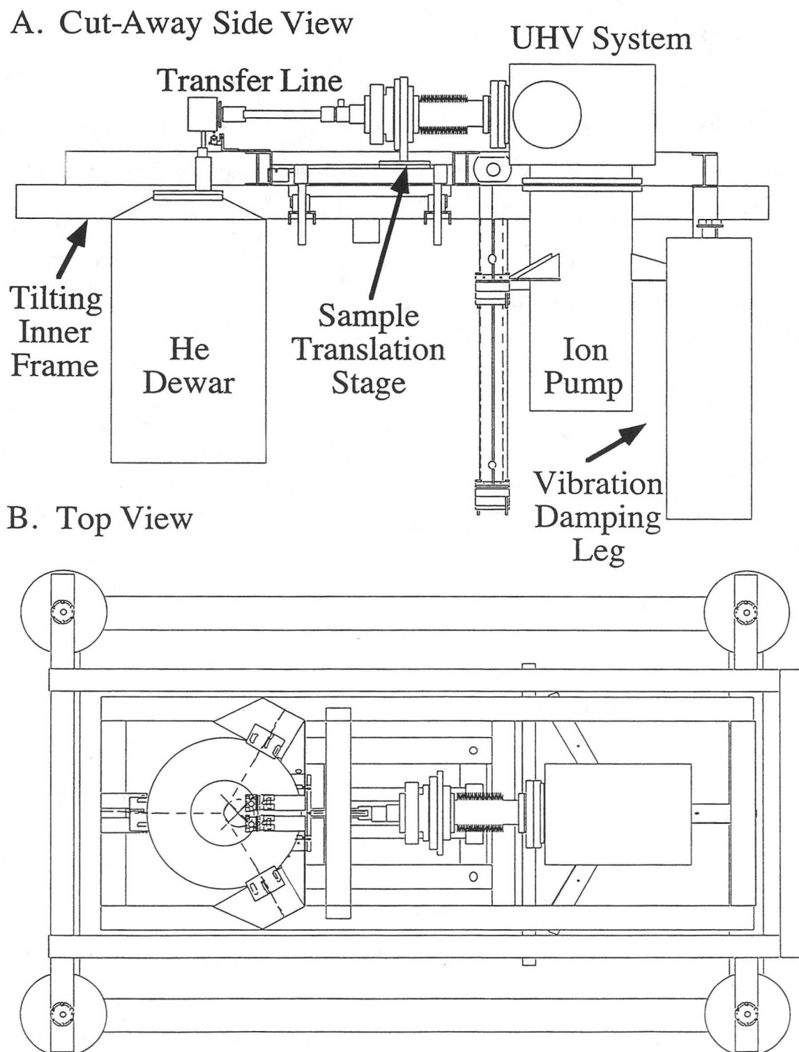
Figure 13.1 Diagram of the Complete System
