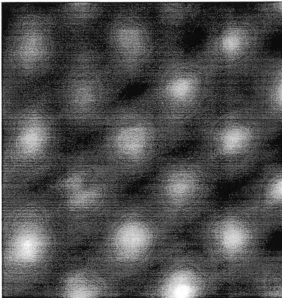
Figure 7.2 A Topographic STM Image of the c(2 \times 2) Structure
