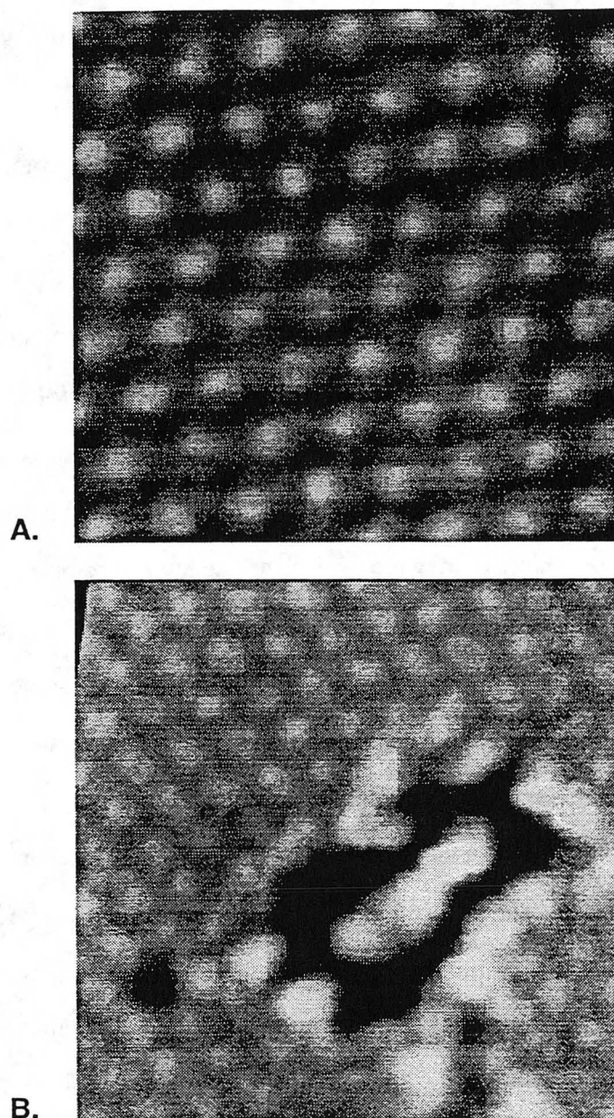
Figure 10.2 STM Images of the CO Induced Reordering of Sulfur
