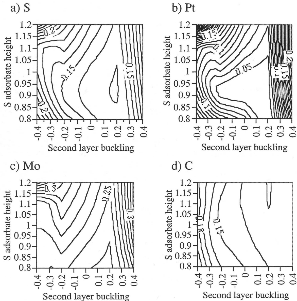
Figure 8.10 Fit Of The Experimental Data To Theory
