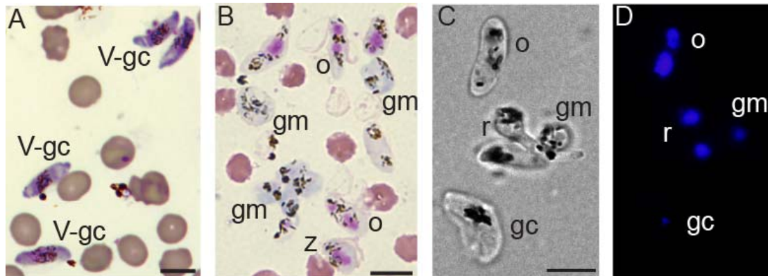
Figure 2.3 Leukostat-stained light micrographs of in vitro -cultivated P. falciparum sexual stage parasites.
