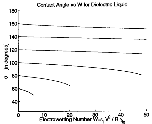
FIG. 6. For a dielectric liquid atop a conducting solid, this plot shows the contact angle dependence on the electro-wetting number W = \epsilon_l V^2 / R\gamma_{lg} for six nominal (zero voltage) contact angles. The analysis above predicts that the drop shape will snap-to complete wetting past some critical electro-wetting number W^* . The predicted snap-to limit W^* is within the plot range for the three bottom curves. Three cautions are necessary: first, the shown snap-to situation for the bottom three curves corresponds to a very high electric field (the drop is thin and the voltage V is high); second, the fit for a_{de}(\theta) used to generate these results does not hold for \theta < 26^\circ ; third, we suspect that other physical effects, like electrolysis, will become active at high V /low \theta , and this snap-to total wetting will not occur.
