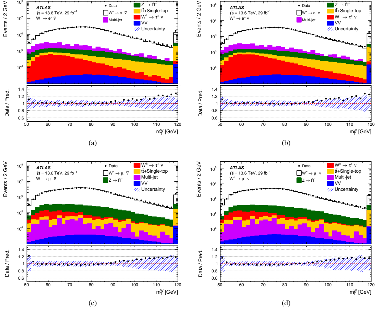
Figure 2: Comparison of data (dots) and predictions (histograms) for the m_T^W distributions in the (a) W^- \rightarrow e^- \bar{\nu} , (b) W^+ \rightarrow e^+ \nu , (c) W^- \rightarrow \mu^- \bar{\nu} , and (d) W^+ \rightarrow \mu^+ \nu channels. The hashed band in the ratio plot denotes the total systematic uncertainty in the prediction. The rightmost bins contain the overflow events.
