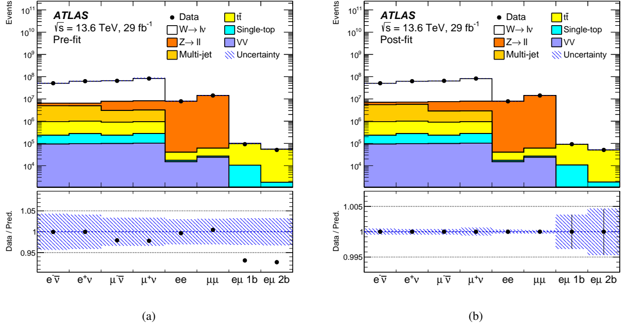
Figure 3: Comparison of the number of data events in each channel (dots) with the predictions (stacked histograms) shown (a) before and (b) after the fits. The dashed error band in the pre-fit figure gives the total systematic uncertainty before the fit, while in the post-fit figure, it represents the statistical uncertainty derived from the fit.
