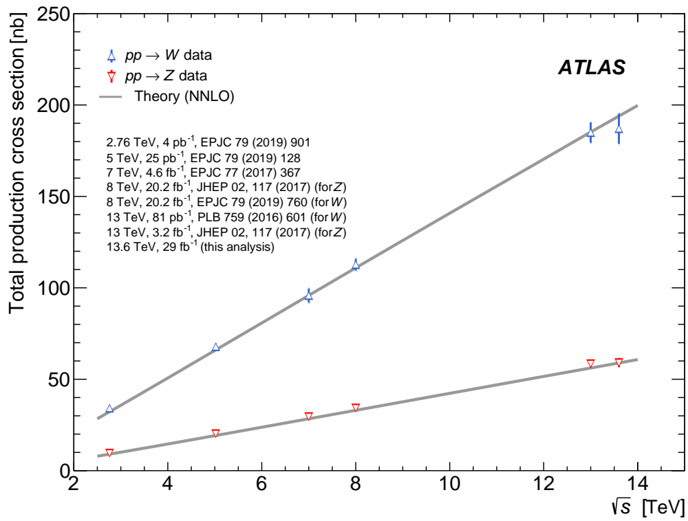
Figure 5: The measured W and Z boson total production cross sections in the leptonic decay channel at different values of centre-of-mass energy. For comparison, the central values of the NNLO predictions based on the CT14NNLO PDF set are included.
