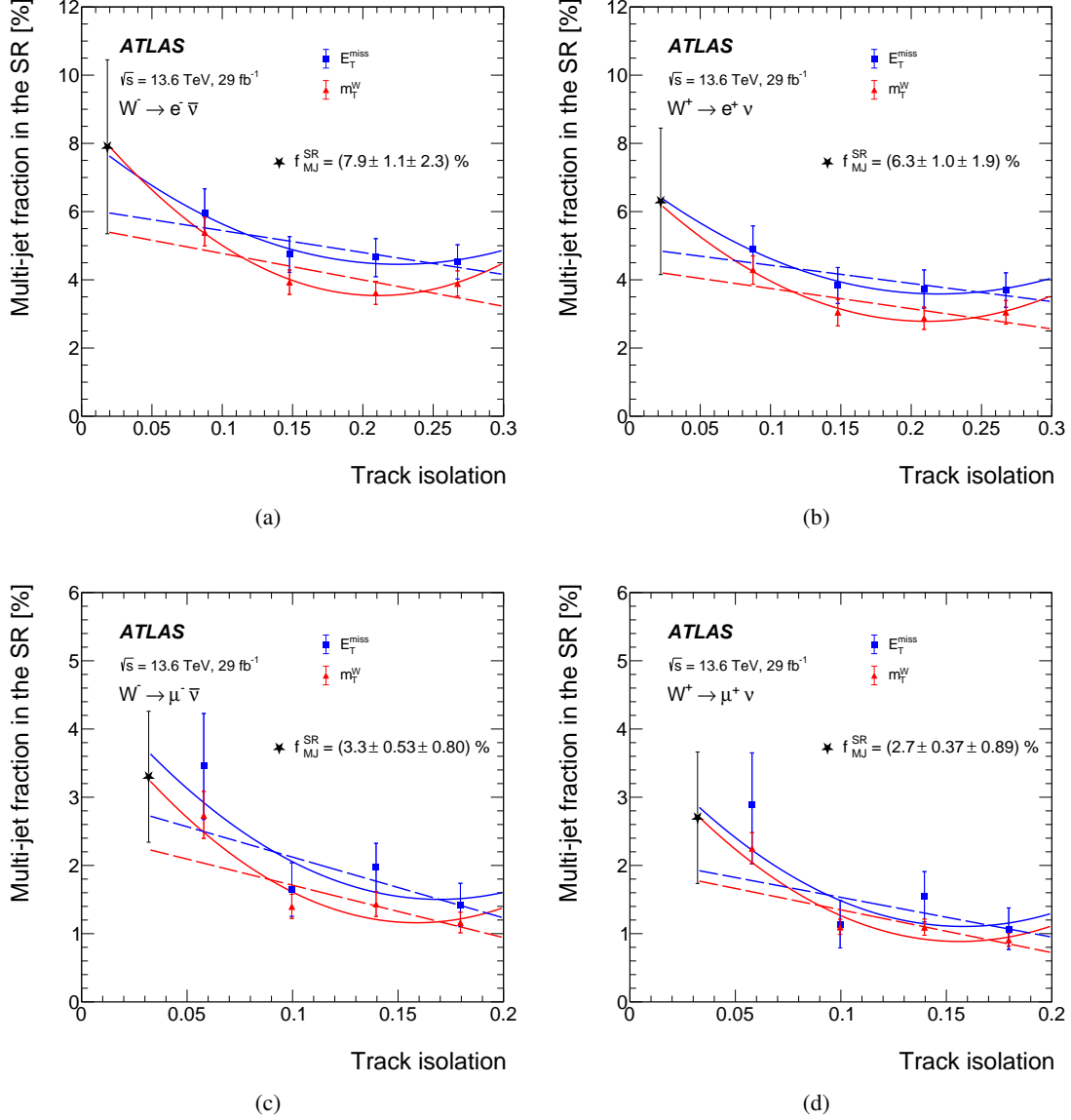
Figure 1: Relative multi-jet yield in the SR as a function of the track isolation variable for the (a) W^- \rightarrow e^- \bar{\nu} , (b) W^+ \rightarrow e^+ \nu , (c) W^- \rightarrow \mu^- \bar{\nu} , and (d) W^+ \rightarrow \mu^+ \nu channels, shown with squares and triangles, respectively for the E_T^{\text{miss}} and m_T^W input measurements. The curves represent the extrapolation of the points to the SR using a quadratic function (solid curves) or a linear function (dashed lines). The x -axis corresponds to the position of the average of a track-isolation slice in the track isolation. The star represents the final MJ fraction ( f_{\text{MJ}}^{\text{SR}} ) and is calculated using the combined average of the quadratic fits in each channel. The first uncertainty corresponds to the combined uncertainty including the difference between the m_T^W and E_T^{\text{miss}} quadratic fits, while the second uncertainty is due to the difference between linear and quadratic fit results.
