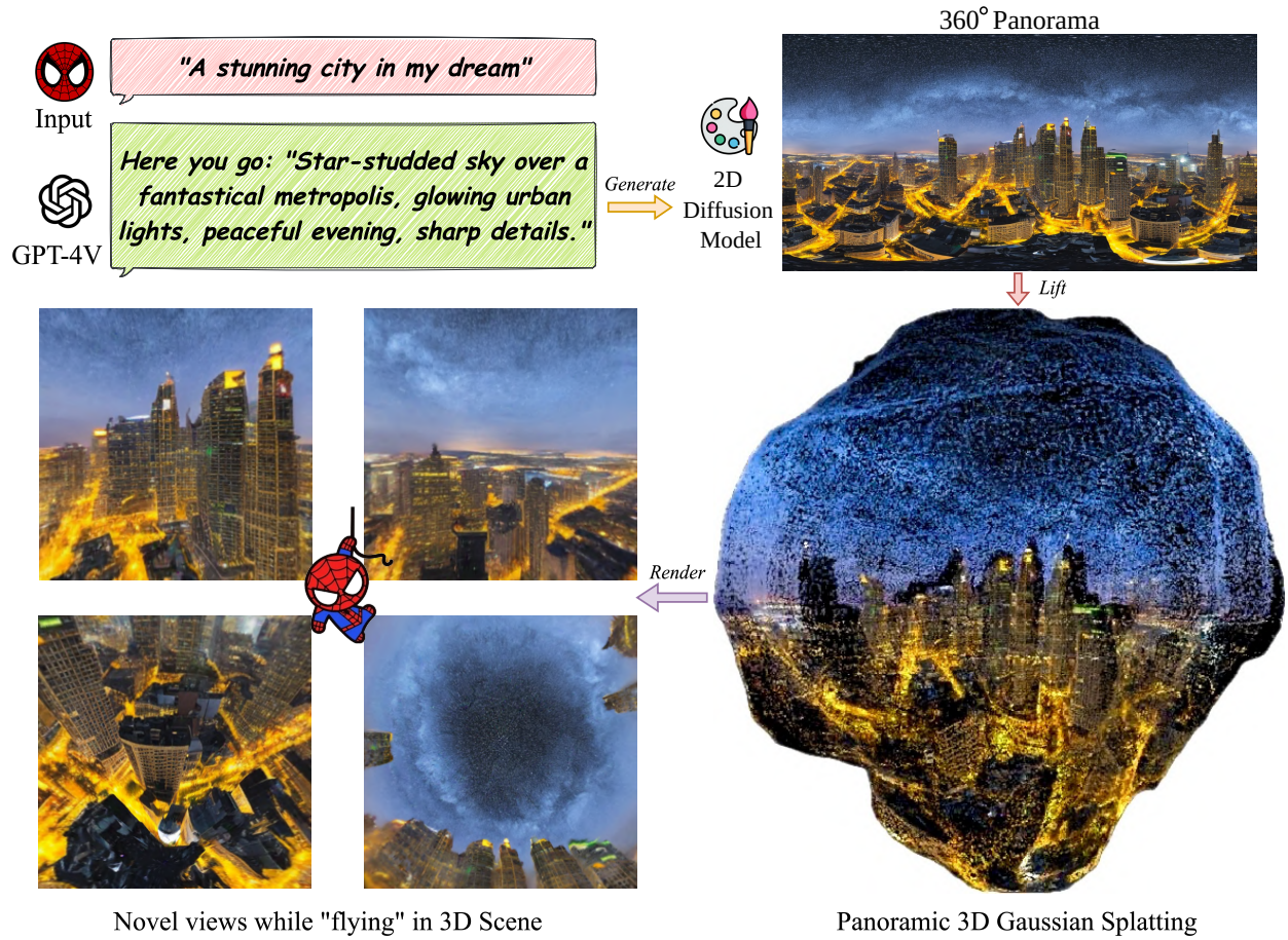
Figure 3.1: DreamScene360 . We introduce a 3D scene generation pipeline that creates immersive scenes with full 360° coverage from text prompts of any level of specificity.
