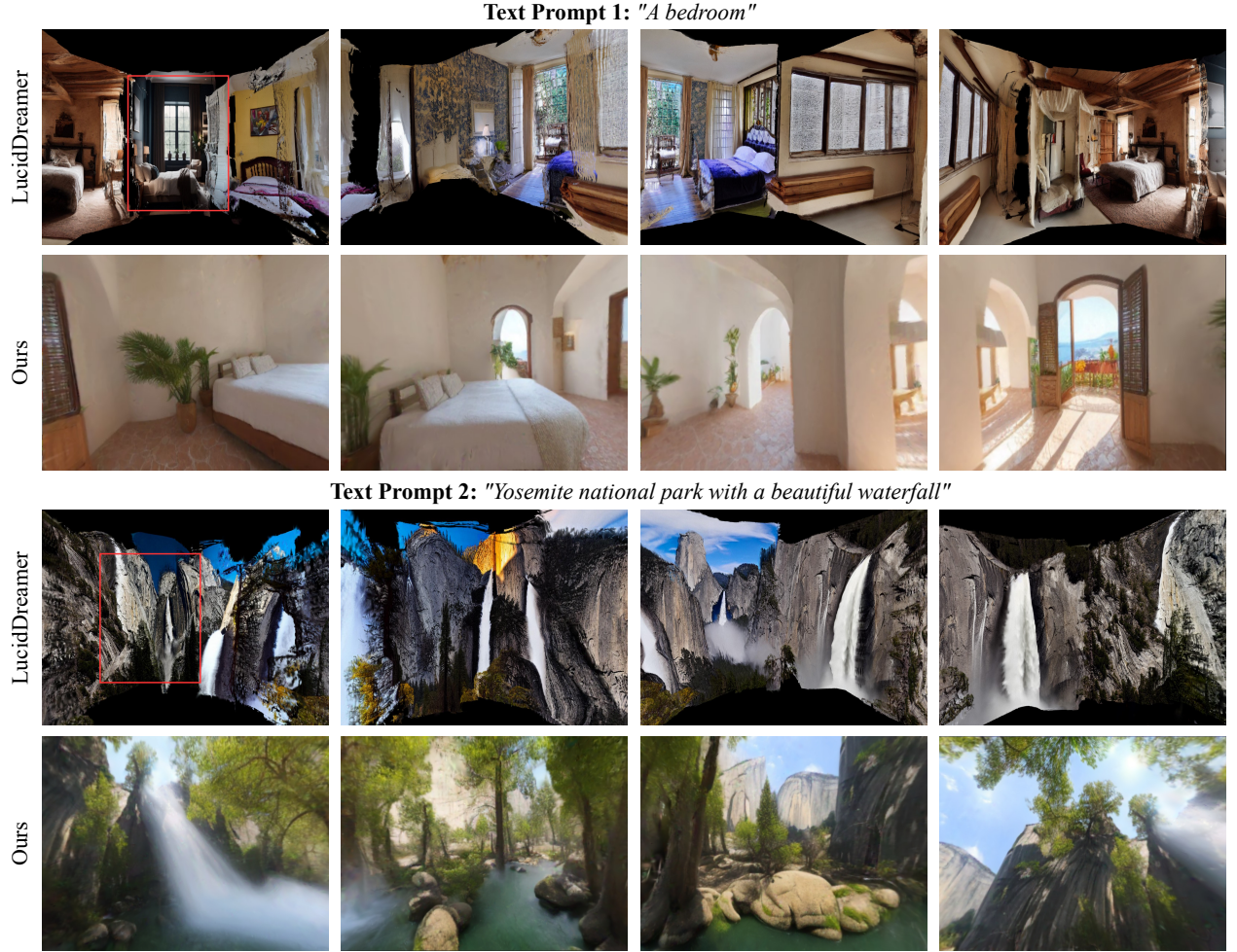
Figure 3.4: Visual Comparisons. We showcase 360° 3D scene generation. In each row, from left to right, displays novel views as the camera undergoes clockwise rotation in yaw, accompanied by slight random rotations in pitch and random translations. LucidDreamer [CLN23] hallucinates novel views from a conditioned image (indicated by a red bounding box) but lacks global semantic, stylized, and geometric consistency. In contrast, our method provides complete 360° coverage without any blind spots (black areas in baseline results), and shows globally consistent semantics.
