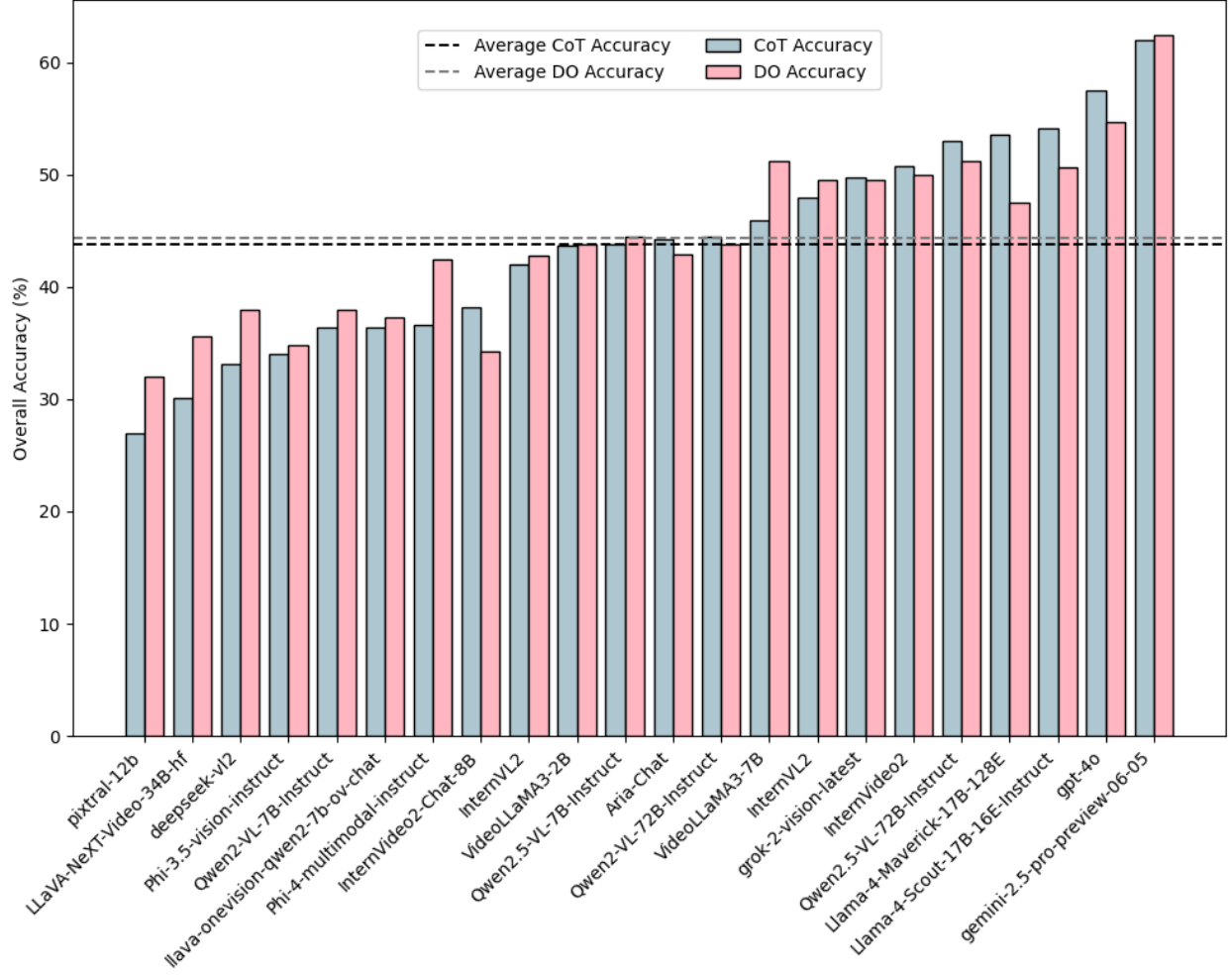
Figure 5.6: Comparison of CoT and DO Accuracy Across Models. Accuracy comparison between Chain-of-Thought (CoT) and Direct Output (DO) prompting across VLMs.
