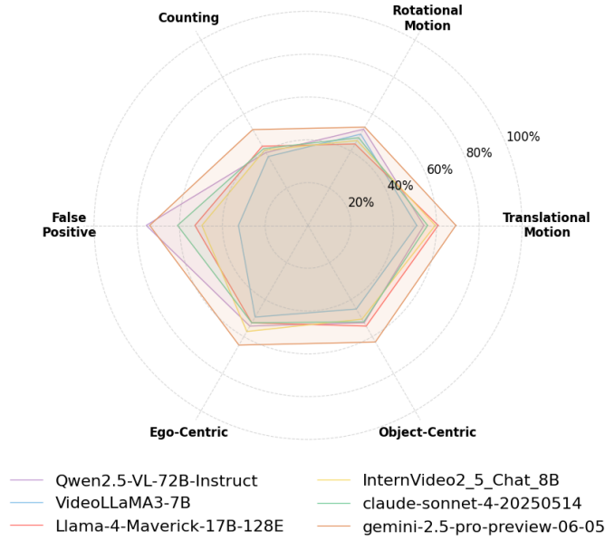
Figure 5.5: Comparison of accuracy across types of spatiotemporal questions. Model accuracy is shown only for the six top-performing VLMs.
