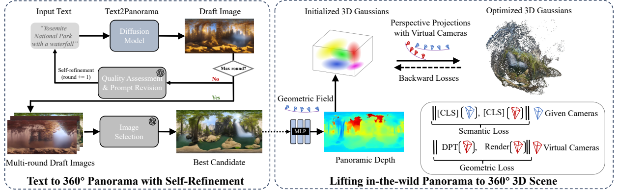
Figure 3.2: Overall Architecture. Beginning with a concise text prompt, we employ a diffusion model to generate a 360° panoramic image. A self-refinement process is employed to produce the optimal 2D candidate panorama. Subsequently, a 3D geometric field is utilized to initialize the Panoramic 3D Gaussians. Throughout this process, both semantic and geometric correspondences are employed as guiding principles for the optimization of the Gaussians, aiming to address and fill the gaps resulting from the single-view input.
