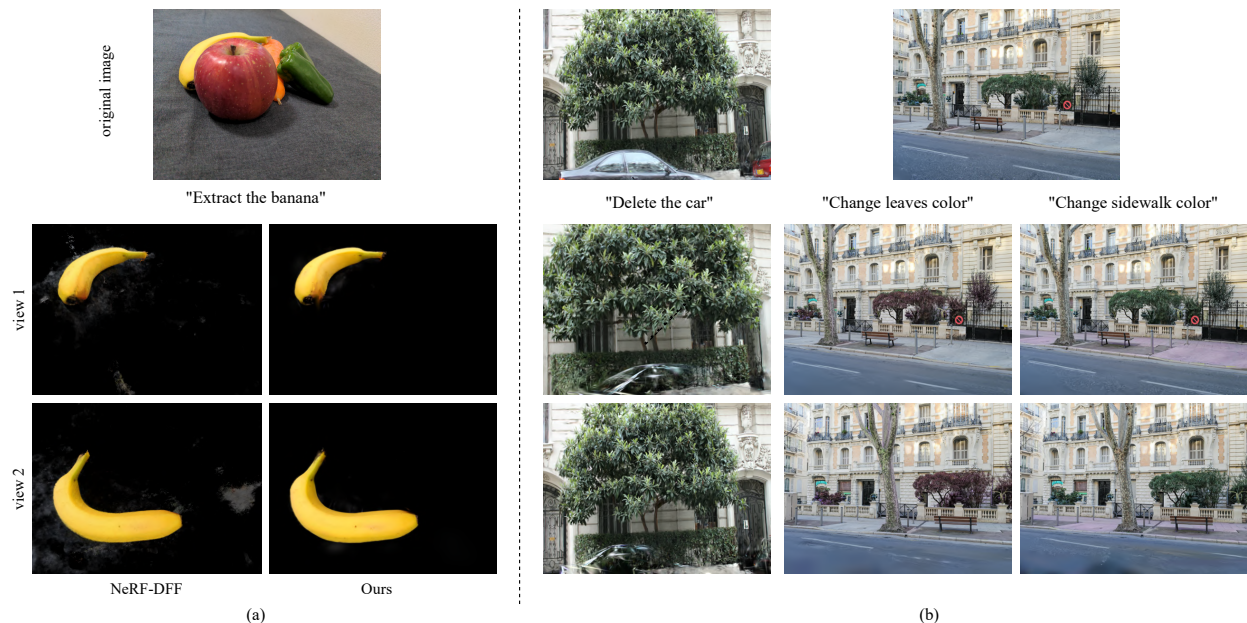
Figure 2.6: Demonstration of results with various language-guided edit operations by querying the 3D feature field and comparison with NeRF-DFF (a) We compare our edit results with NeRF-DFF method on the sample dataset provided by NeRF-DFF [KMS22]. Note that our method outperforms NeRF-DFF method by extracting the entire banana hidden by an apple in the original image and with less floaters in the background. (b) We demonstrate results with deletion and appearance modification on different targets. Note that the car is deleted with background preserved, and the appearance of the leaves changes with the appearance of the stop sign remained the same.
