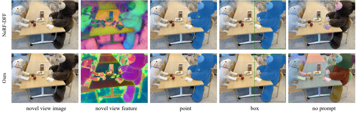
Figure 2.5: Novel view segmentation (SAM) results compared with NeRF-DFF. (Upper) NeRF-DFF method presents lower-quality segmentation masks - note the failure on segmenting the cup from the bear and the coarse-grained mask boundary on the bear’s leg in box-prompted results. (Lower) Our method provides higher-quality masks with more fine-grained segmentation details. Scene from [KKG23].
