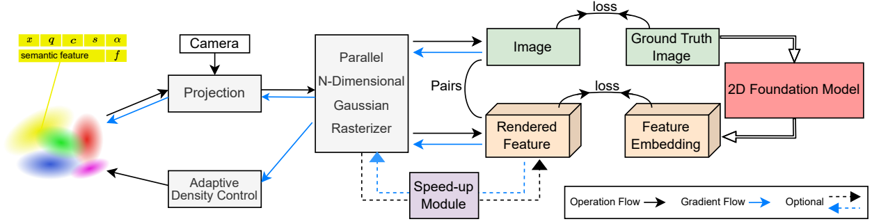
Figure 2.2: An overview of our method. We adopt the same 3D Gaussian initialization from sparse SfM point clouds as utilized in 3DGS, with the addition of an essential attribute: the semantic feature . Our primary innovation lies in the development of a Parallel N-dimensional Gaussian Rasterizer, complemented by a convolutional speed-up module as an optional branch. This configuration is adept at rapidly rendering arbitrarily high-dimensional features without sacrificing downstream performance.
