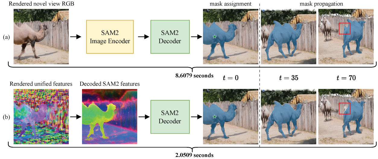
Figure 4.4: Baseline Comparison on SAM2 Inference. We compare segmentation quality and inference speed between (a) the naive RGB-based approach and (b) our feature-based method. Ours achieves comparable segmentation, accurately tracking the object over time, and avoids RGB artifacts (red box region at t = 70 ), while reducing inference time to about 4\times speed-up.
