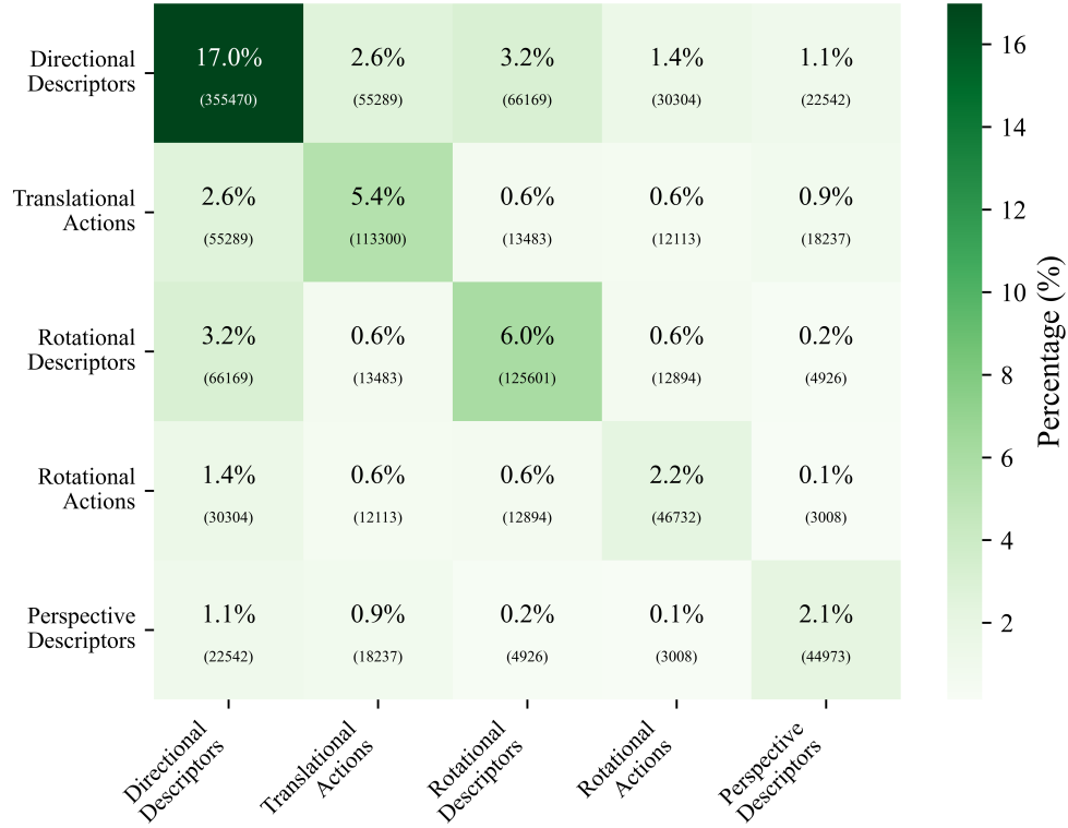
Figure 5.7: Heatmap of Occurances of Spatial-Temporal Terms in popular video SFT datasets.
