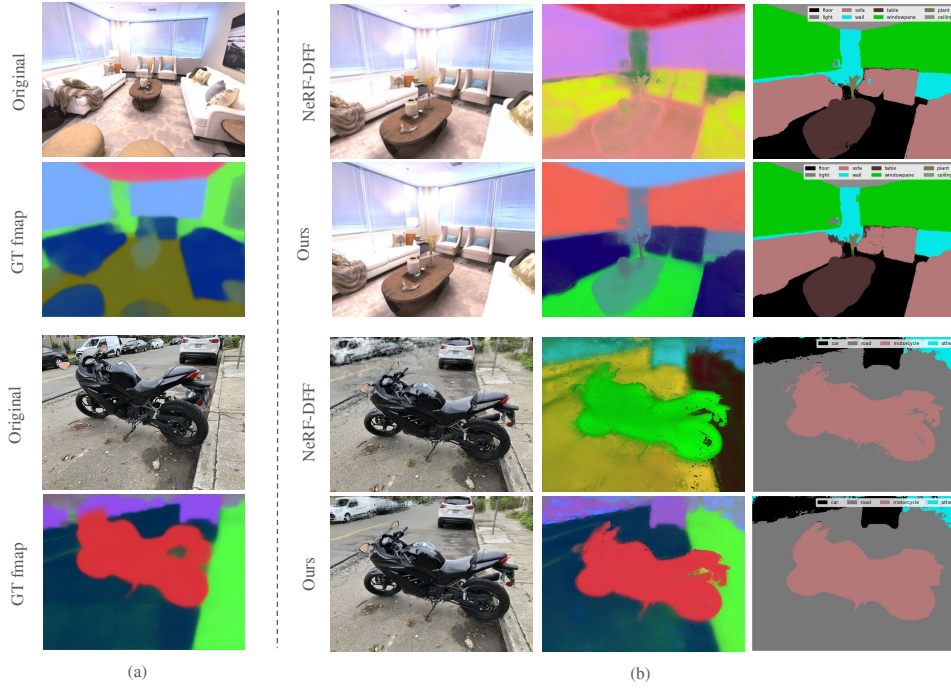
Figure 2.3: Novel view semantic segmentation (LSeg) results on scenes from Replica dataset [SWM19] and LLFF dataset [MSO19]. (a) We show examples of original images in training views together with the ground-truth feature visualizations. (b) We compare the qualitative segmentation results using our Feature 3DGS with the NeRF-DFF [KMS22]. Our inference is 1.66\times faster when rendered feature dim = 128 . Our method demonstrates more fine-grained segmentation results with higher-quality feature maps.
