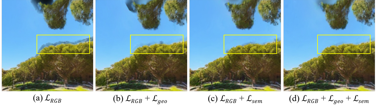
Figure 3.6: Ablation of Optimization Loss. We demonstrate the impact of Semantic and Geometric losses on the synthesized virtual cameras. (a) Utilizing photometric loss on camera views from a rendered panorama induces artifacts when altering rendered camera positions. (b) Implementing Geometric and (c) Semantic regularizations effectively reduces the artifacts originating from invisible views. (d) Integrating both regularizations yields the most optimal outcomes.
