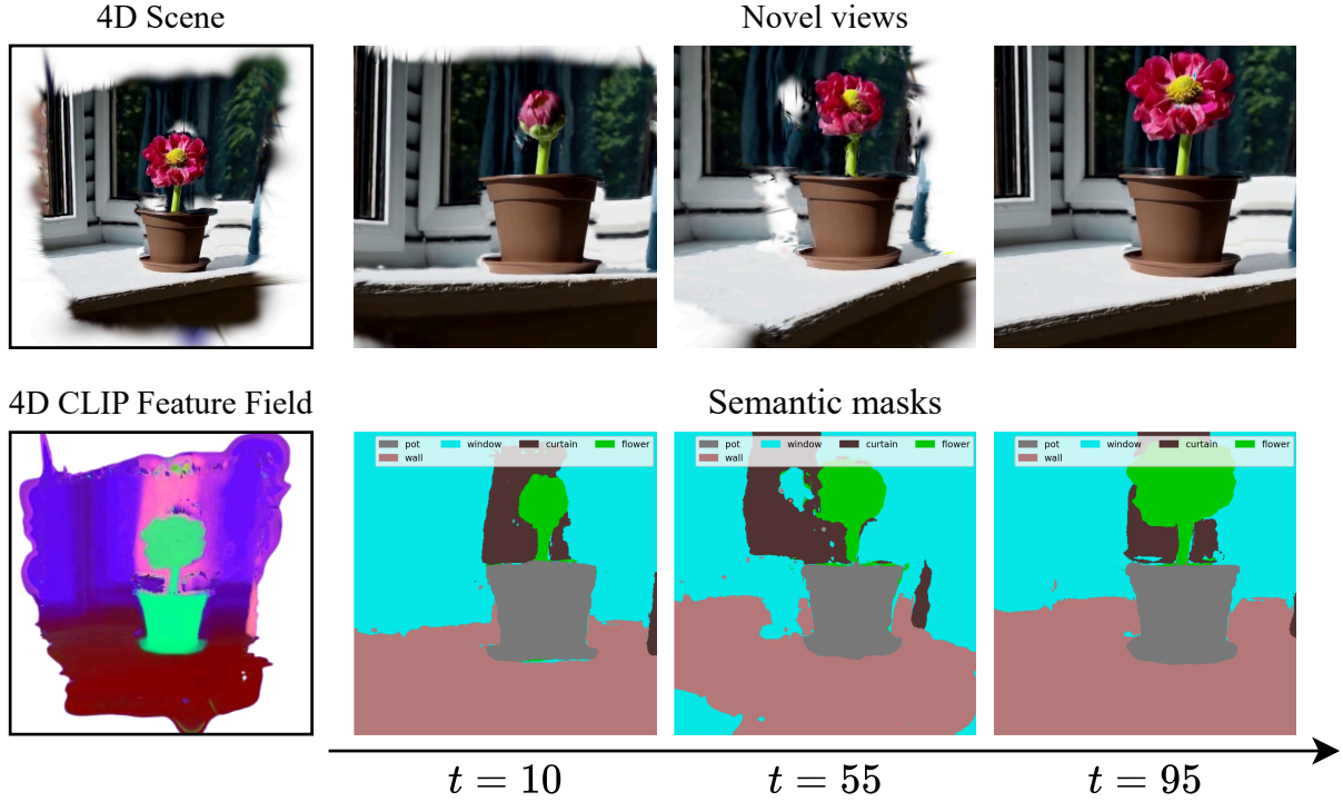
Figure 4.5: Semantic 4D Scene Understanding with CLIP Feature Field. By lifting CLIP-LSeg [LWB22a] features into a 4D feature field, we enable pixel-level semantic segmentation from any view at any timestep. This allows robust 4D scene understanding, even as object appearances change over time—for example, accurately identifying a blooming flower from bud to full bloom across views.
