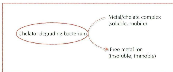
Figure 5.5. Immobilization of radionuclides and heavy metals by enzymatic degradation of organic chelators, such as EDTA and NTA.
