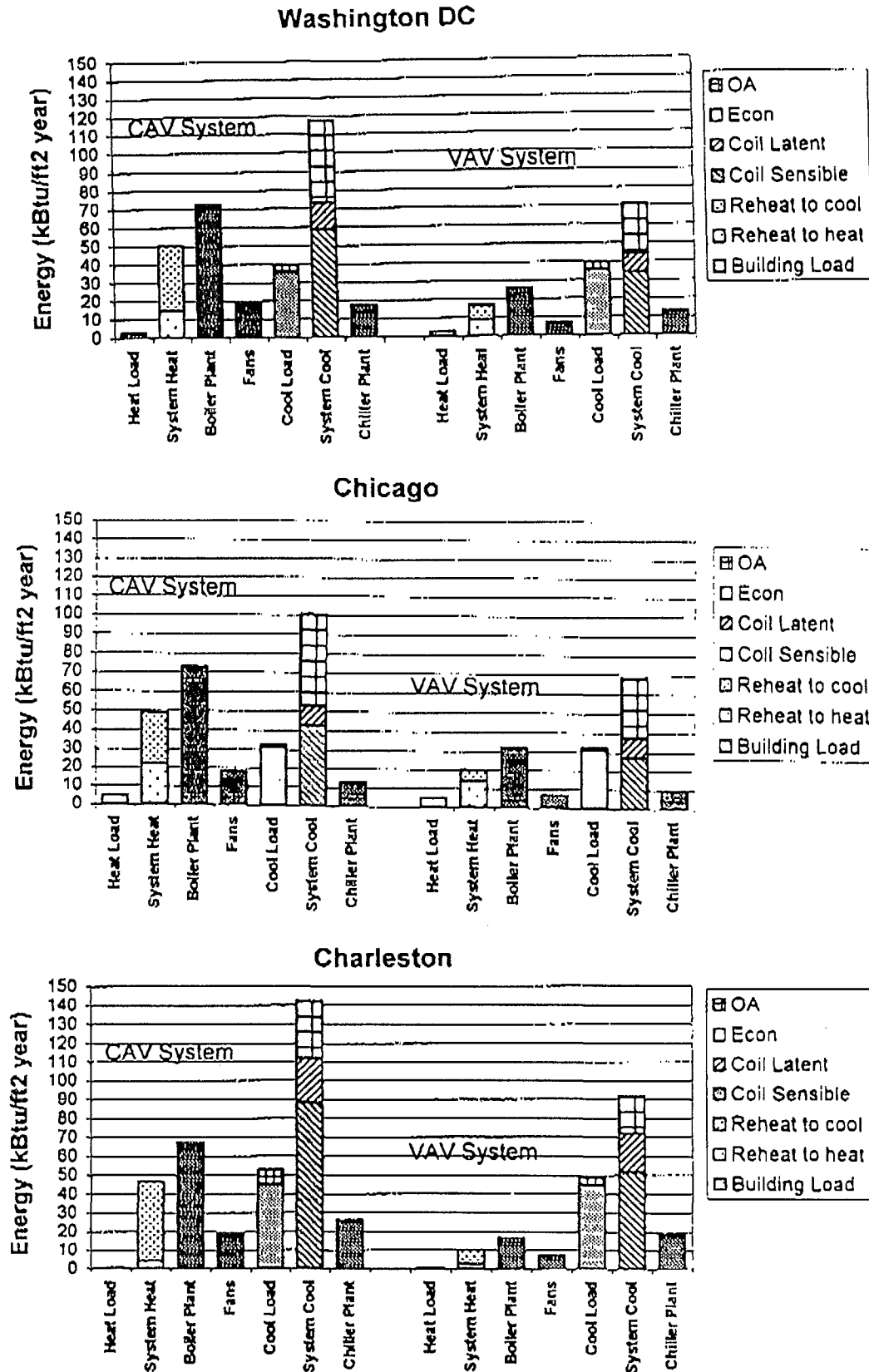
Figure 1. CAV and VAV System Performance Comparison System Serving 15000 ft² Office Building Floor
