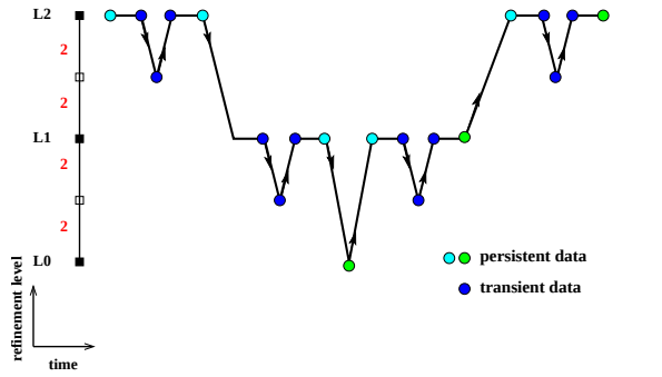
Figure 5. A simple sketch of one multigrid V-cycle. There are three levels of refinement in this grid hierarchy. The refinement ratio is 4 between two adjacent levels. Here, the direction of data flow is indicated by arrows. The small V-cycles are contributed by the mgRelax subroutine, which itself is a multigrid algorithm.
