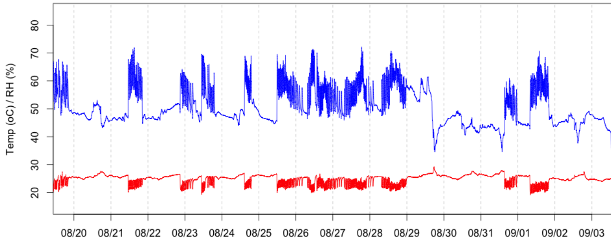
Figure 14 Temperature (in red) and relative humidity (in blue) measured at a supply air grille of the central forced air system in the two pilot homes.
