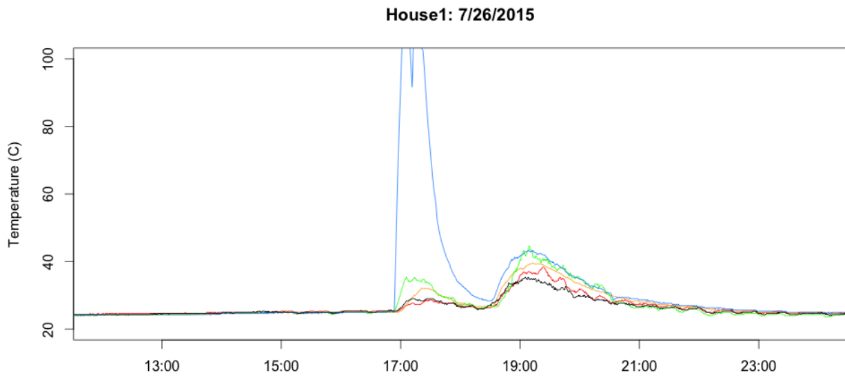
Figure 10 Temperature measured outside of oven (in black) and on cooktop (lines in color). Occupants reported 45 minutes of oven use followed by 1.5 hours of cooktop use on July 22. On July 26, occupants reported 30 minutes of cooktop use followed by 30 minutes of oven use.
