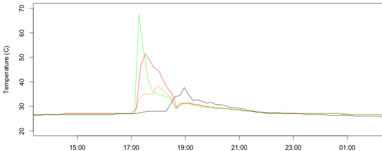
Figure 11 Temperature measured outside of oven (in black) and on cooktop (lines in color). Occupants reported 30 minutes of cooktop use followed by 45 minutes of oven use on August 26. On August 29, occupants reported 40 minutes of cooktop use followed by 30 minutes of oven use.
