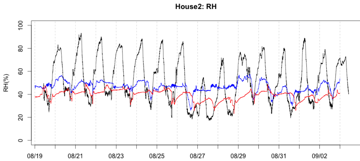
Figure 13 Temperature and relative humidity measured outdoors (black) and indoors (living room in red, master bedroom in blue).
