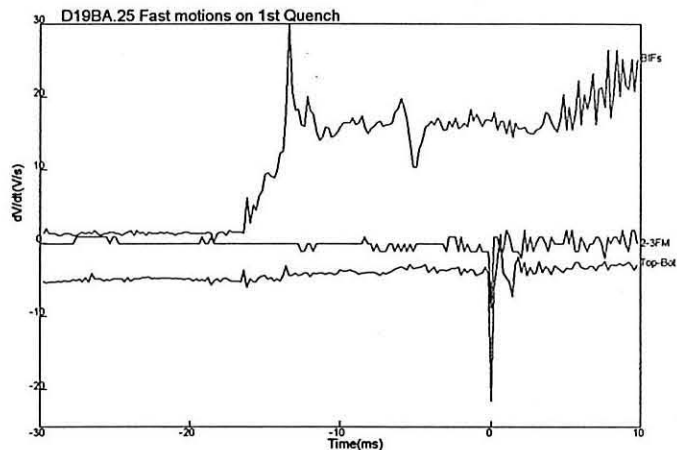
Fig. 6. 1st quench (#24): The largest fast-motion transient produced the stop-trigger ( t = 0 ) but occurred 17 ms after quench-initiation (BIFs @ t = -17 ms.). A smaller one was coincident with quench onset.
