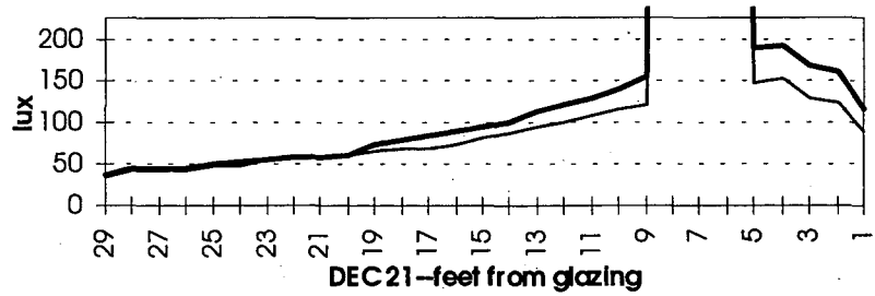
Figure 11. Illuminance distribution at 30 inches above the floor with holographic glazing with 75.6^\circ acceptance and 18^\circ diffraction angles (bold line) versus clear glazing (thin line).
