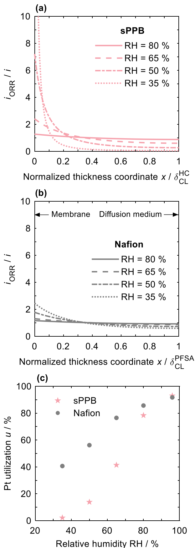
Fig. 2. Distribution of i_{ORR} normalized to an average current density i = 50 \text{ mA cm}^{-2} for (a) a fully sPPB-based CCM ( I/C = 0.2 ) or (b) a fully Nafion-based CCM ( I/C = 0.8 ) as a function of the cathode CL thickness coordinate x (i.e., x = 0 at the membrane/CL interface and x = \delta_{CL} at the CL/gas diffusion media interface). For better comparison, x was normalized to the thickness \delta_{CL} of the cathode CL. (c) Calculated protonic resistance-induced Pt utilization u over RH for sPPB- and Nafion-based CCMs at 80^\circ \text{C} .
