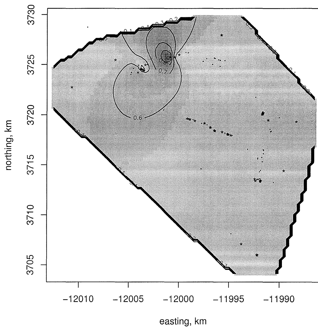
FIGURE 2: Kriging surface for user id 6. The surface was computed using the named (starred) activities. The small dots represent unlabeled points. The dark areas represent higher expected frequencies, and the white areas lower frequencies.
