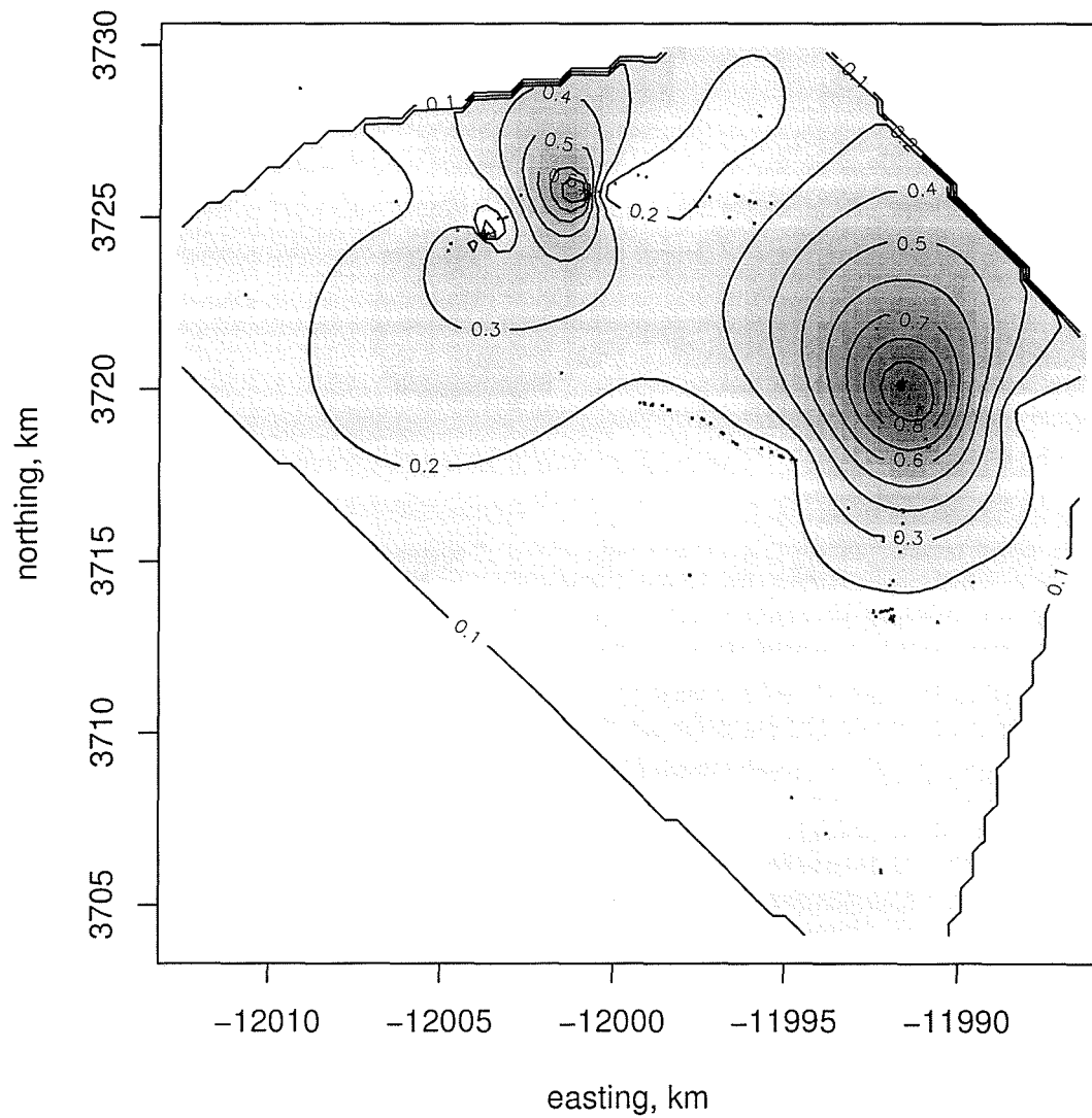
FIGURE 3: Kriging surface for user id 6 activity 1. The stars are activity 1 observations, while the points are both labeled and unlabeled destinations. Compare areas of high and low expected frequency to the “any activity” surface of figure 2.
