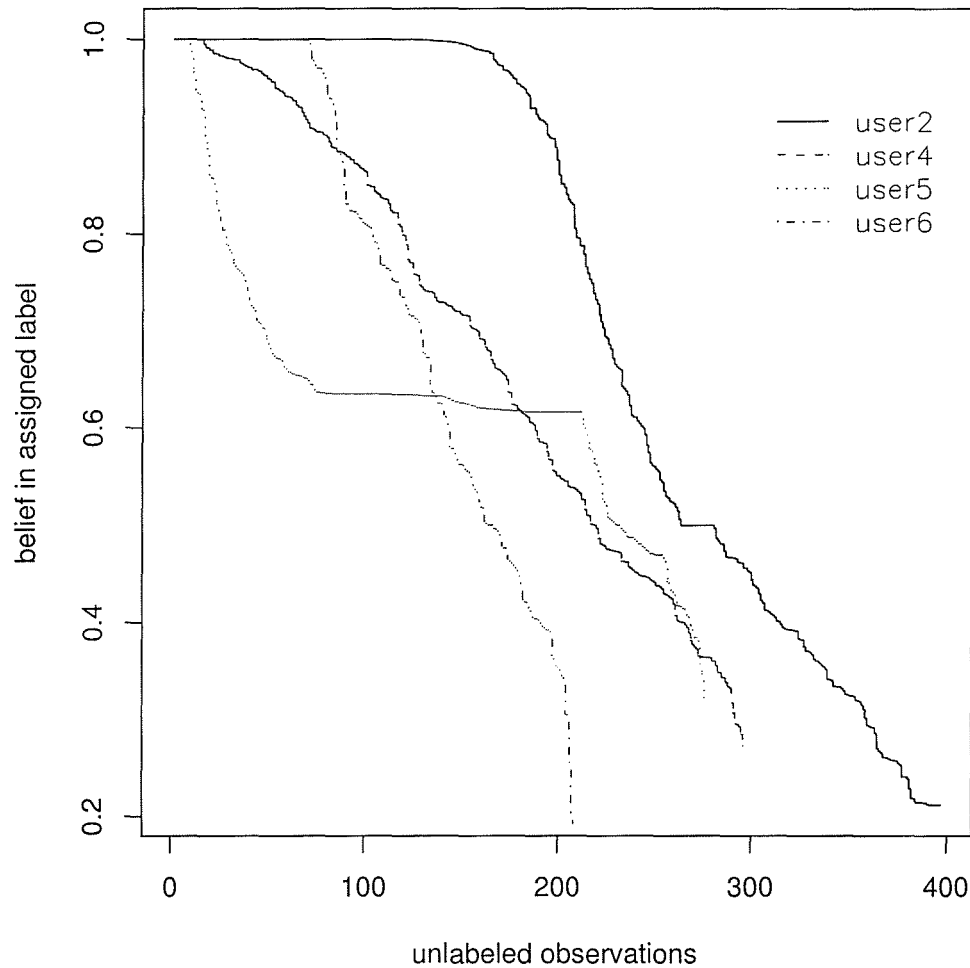
FIGURE 4: Probabilities of the most likely activity labels assigned to each unknown activity for each of four pilot survey volunteers, given the responses to the on-line survey. The more activities are entered, the more refined the activity-specific kriging surfaces, and the higher the corresponding belief associated with unlabeled activities. (Note that activities have been resorted from best prediction to worst prediction for each respondent.)
